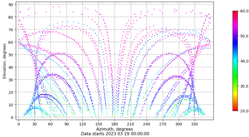
Azimuth-elevation plot for station TALV. Signal to Noise S1C Data file TALV00ESP_R_2023078.xtr
