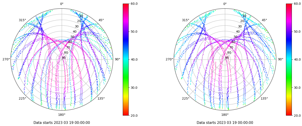
Skyplot for station TALV. Signal to Noise S1C Data file TALV00ESP_R_2023078.xtr Skyplot for station TALV. Signal to Noise S2P Data file TALV00ESP_R_2023078.xtr
