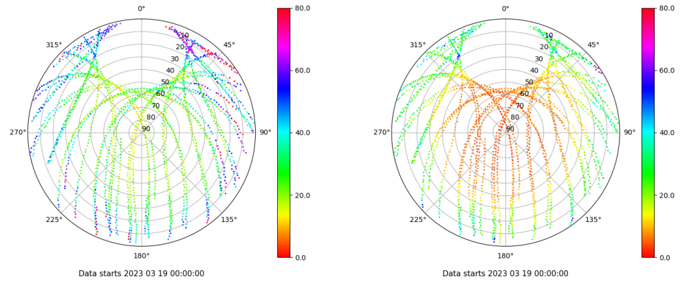
Skyplot for station TALV. Parameter M1C Data file TALV00ESP_R_2023078.xtr Skyplot for station TALV. Parameter M2P Data file TALV00ESP_R_2023078.xtr
