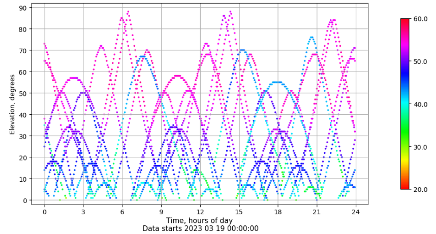
Time-elevation plot for station TALV. Signal to Noise S1C Data file TALV00ESP_R_2023078.xtr
