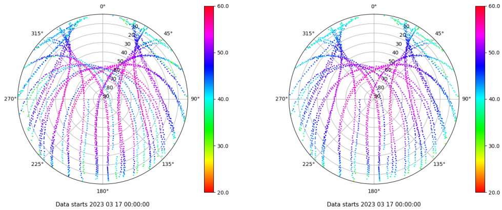
Skyplot for station TALV. Signal to Noise S1C Data file TALV00ESP_R_2023076.xtr Skyplot for station TALV. Signal to Noise S2P Data file TALV00ESP_R_2023076.xtr
