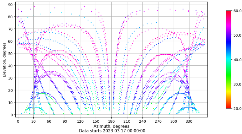
Azimuth-elevation plot for station TALV. Signal to Noise S1C Data file TALV00ESP_R_2023076.xtr
