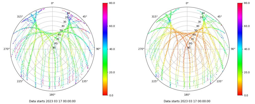
Skyplot for station TALV. Parameter M1C Data file TALV00ESP_R_2023076.xtr Skyplot for station TALV. Parameter M2P Data file TALV00ESP_R_2023076.xtr
