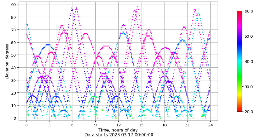
Time-elevation plot for station TALV. Signal to Noise S1C Data file TALV00ESP_R_2023076.xtr
