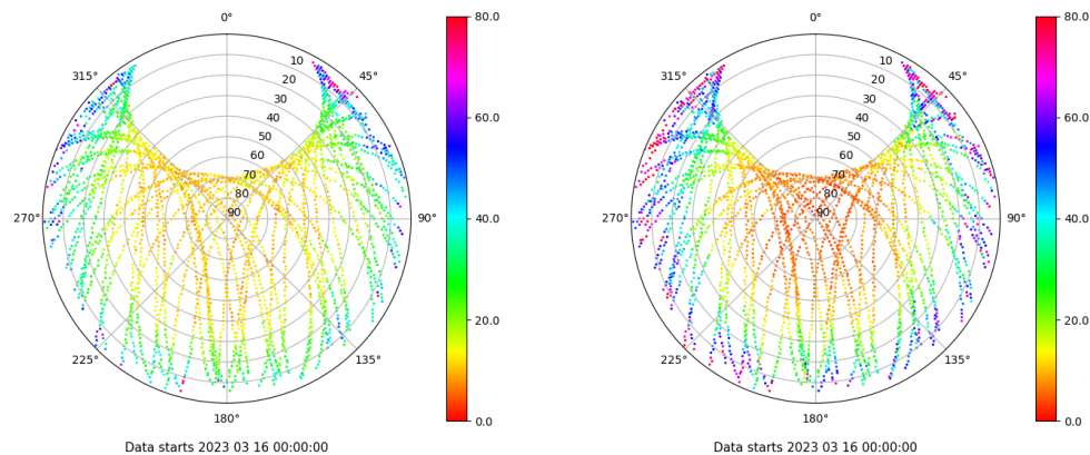
Skyplot for station TALV. Parameter M1C Data file TALV00ESP_R_2023075.xtr Skyplot for station TALV. Parameter M2W Data file TALV00ESP_R_2023075.xtr
