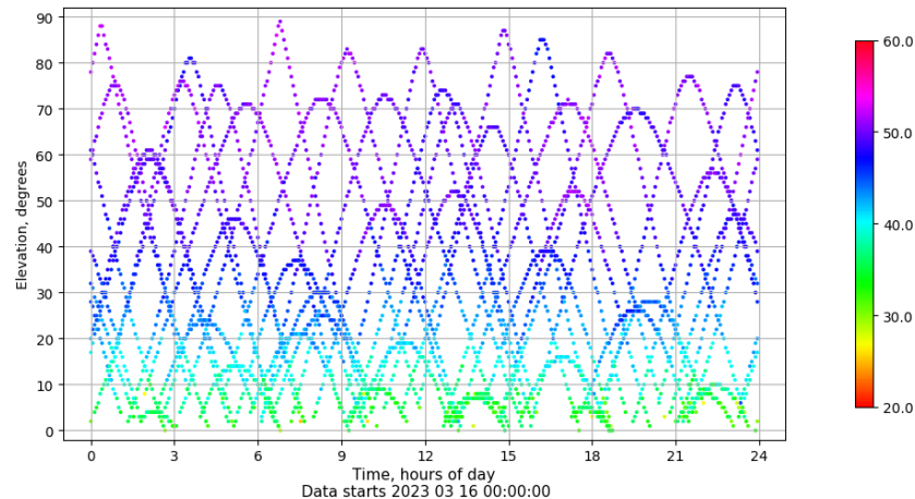
Time-elevation plot for station TALV. Signal to Noise S1C Data file TALV00ESP_R_2023075.xtr
