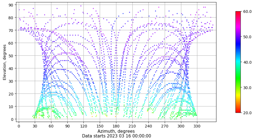
Azimuth-elevation plot for station TALV. Signal to Noise S1C Data file TALV00ESP_R_2023075.xtr
