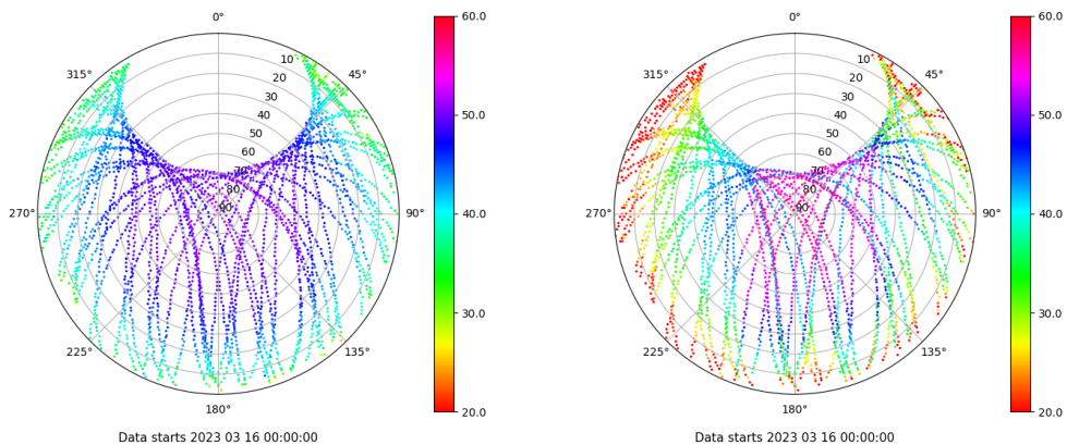
Skyplot for station TALV. Signal to Noise S1C Data file TALV00ESP_R_2023075.xtr Skyplot for station TALV. Signal to Noise S2W Data file TALV00ESP_R_2023075.xtr
