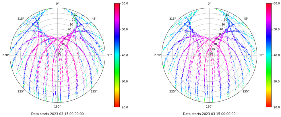
Skyplot for station TALV. Signal to Noise S1C Data file TALV00ESP_R_2023074.xtr Skyplot for station TALV. Signal to Noise S2P Data file TALV00ESP_R_2023074.xtr
