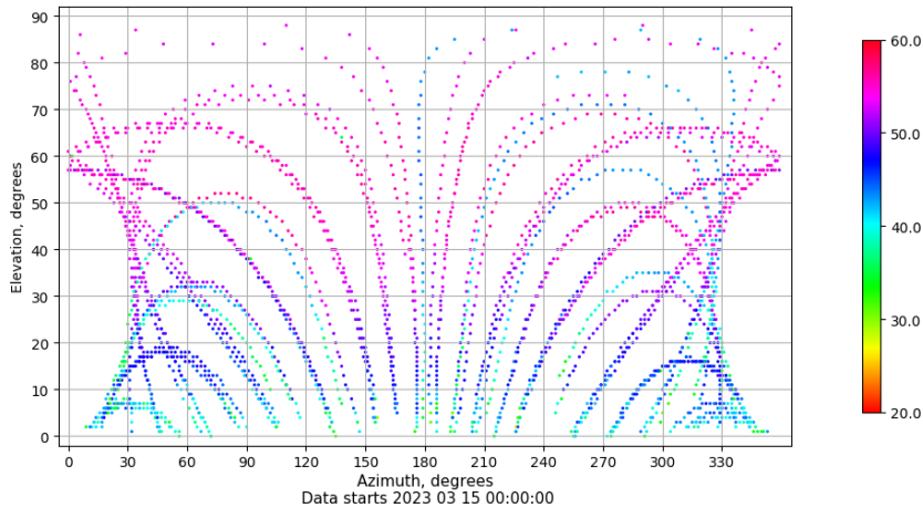
Azimuth-elevation plot for station TALV. Signal to Noise S1C Data file TALV00ESP_R_2023074.xtr
