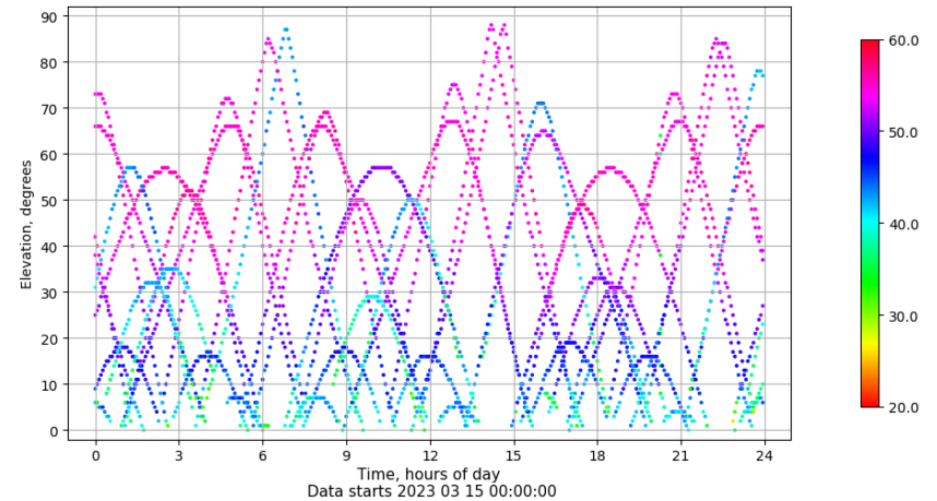
Time-elevation plot for station TALV. Signal to Noise S1C Data file TALV00ESP_R_2023074.xtr
