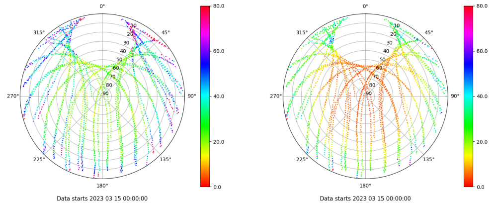
Skyplot for station TALV. Parameter M1C Data file TALV00ESP_R_2023074.xtr Skyplot for station TALV. Parameter M2P Data file TALV00ESP_R_2023074.xtr
