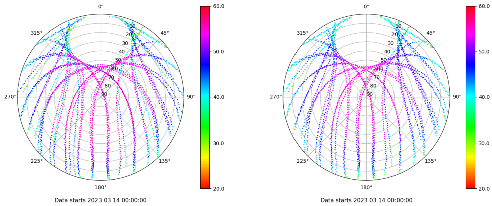
Skyplot for station TALV. Signal to Noise S1C Data file TALV00ESP_R_2023073.xtr Skyplot for station TALV. Signal to Noise S2P Data file TALV00ESP_R_2023073.xtr
