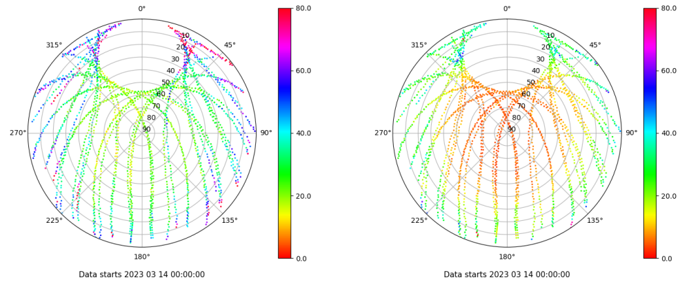
Skyplot for station TALV. Parameter M1C Data file TALV00ESP_R_2023073.xtr Skyplot for station TALV. Parameter M2P Data file TALV00ESP_R_2023073.xtr
