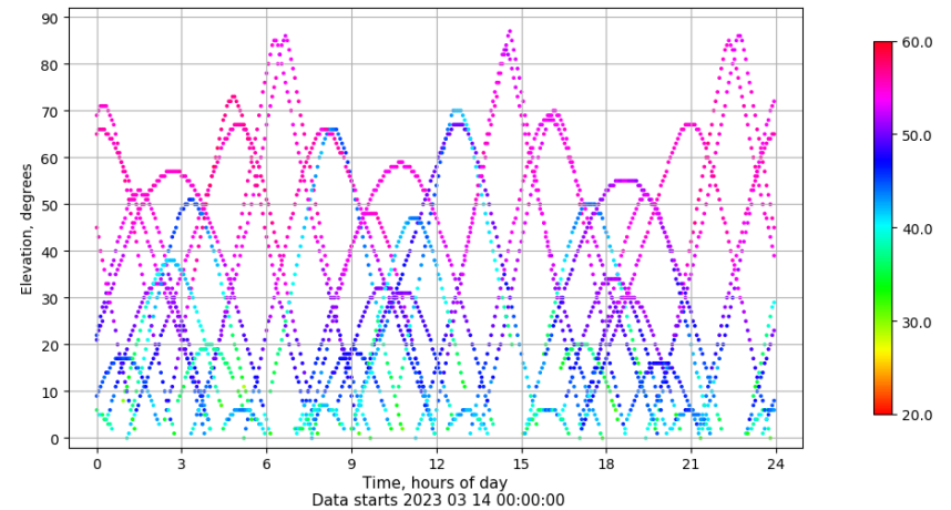
Time-elevation plot for station TALV. Signal to Noise S1C Data file TALV00ESP_R_2023073.xtr
