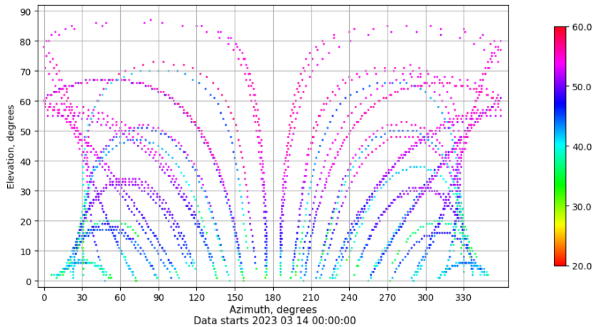
Azimuth-elevation plot for station TALV. Signal to Noise S1C Data file TALV00ESP_R_2023073.xtr
