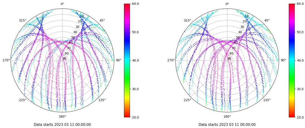
Skyplot for station TALV. Signal to Noise S1C Data file TALV00ESP_R_2023070.xtr Skyplot for station TALV. Signal to Noise S2P Data file TALV00ESP_R_2023070.xtr
