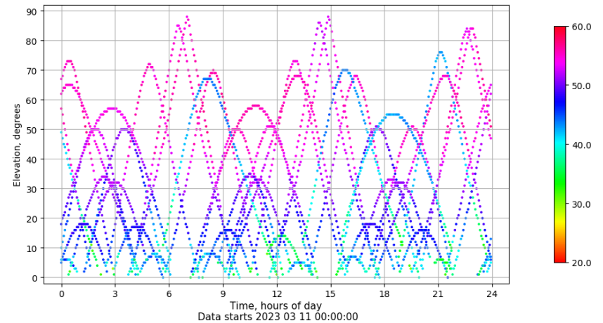
Time-elevation plot for station TALV. Signal to Noise S1C Data file TALV00ESP_R_2023070.xtr
