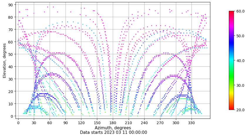
Azimuth-elevation plot for station TALV. Signal to Noise S1C Data file TALV00ESP_R_2023070.xtr
