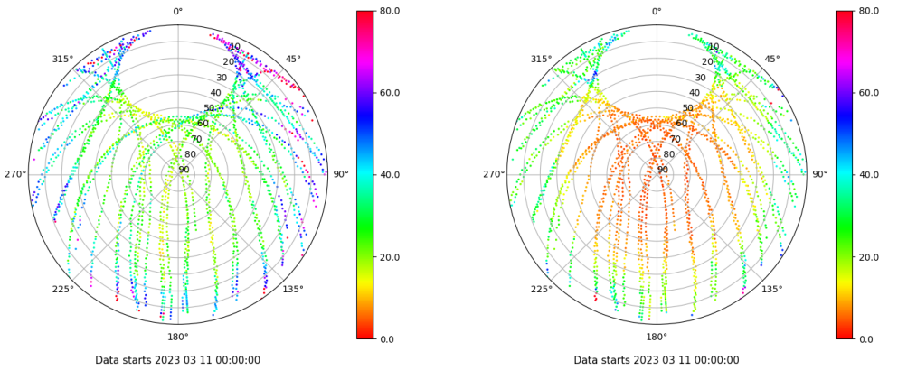
Skyplot for station TALV. Parameter M1C Data file TALV00ESP_R_2023070.xtr Skyplot for station TALV. Parameter M2P Data file TALV00ESP_R_2023070.xtr
