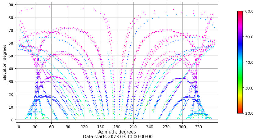
Azimuth-elevation plot for station TALV. Signal to Noise S1C Data file TALV00ESP_R_2023069.xtr
