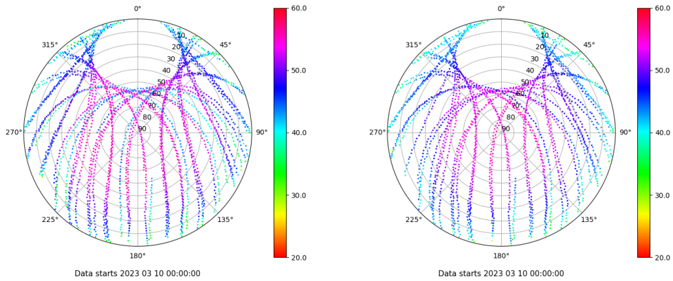
Skyplot for station TALV. Signal to Noise S1C Data file TALV00ESP_R_2023069.xtr Skyplot for station TALV. Signal to Noise S2P Data file TALV00ESP_R_2023069.xtr
