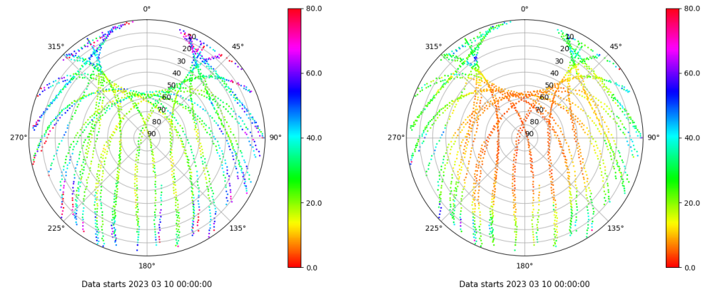
Skyplot for station TALV. Parameter M1C Data file TALV00ESP_R_2023069.xtr Skyplot for station TALV. Parameter M2P Data file TALV00ESP_R_2023069.xtr
