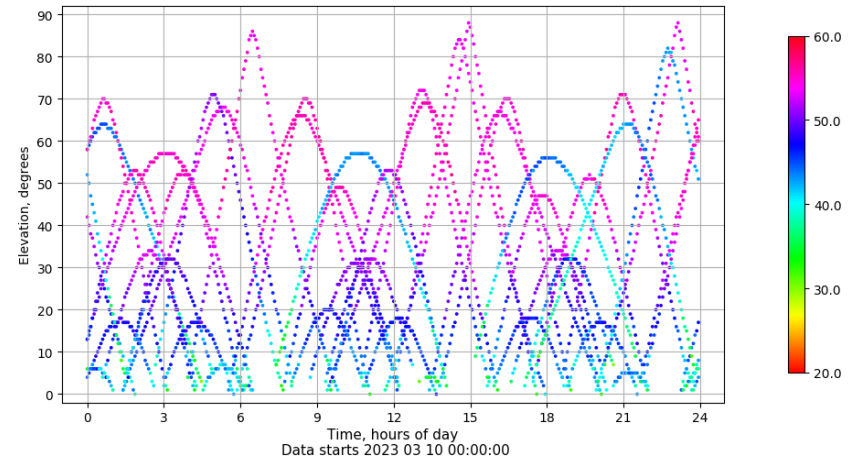
Time-elevation plot for station TALV. Signal to Noise S1C Data file TALV00ESP_R_2023069.xtr
