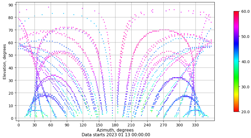
Azimuth-elevation plot for station TALV. Signal to Noise S1C Data file TALV00ESP_R_2023013.xtr
