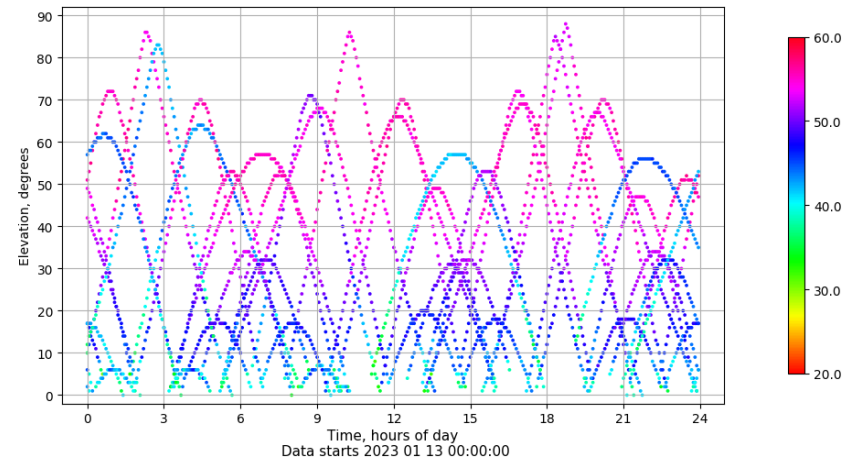
Time-elevation plot for station TALV. Signal to Noise S1C Data file TALV00ESP_R_2023013.xtr
