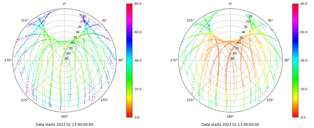
Skyplot for station TALV. Parameter M1C Data file TALV00ESP_R_2023013.xtr Skyplot for station TALV. Parameter M2P Data file TALV00ESP_R_2023013.xtr
