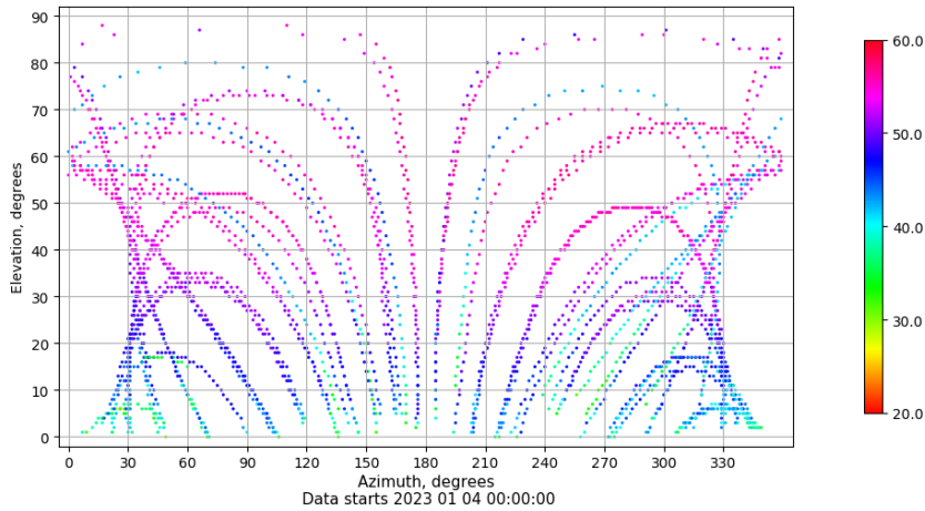
Azimuth-elevation plot for station TALV. Signal to Noise S1C Data file TALV00ESP_R_2023004.xtr
