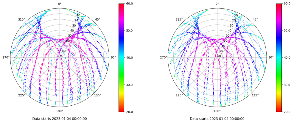
Skyplot for station TALV. Signal to Noise S1C Data file TALV00ESP_R_2023004.xtr Skyplot for station TALV. Signal to Noise S2P Data file TALV00ESP_R_2023004.xtr
