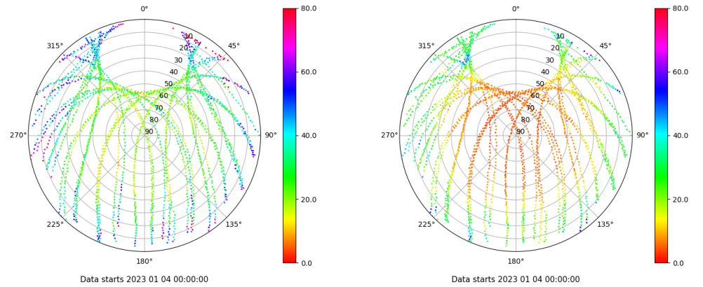
Skyplot for station TALV. Parameter M1C Data file TALV00ESP_R_2023004.xtr Skyplot for station TALV. Parameter M2P Data file TALV00ESP_R_2023004.xtr
