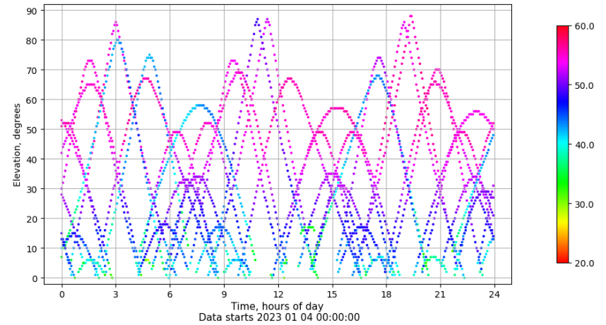
Time-elevation plot for station TALV. Signal to Noise S1C Data file TALV00ESP_R_2023004.xtr
