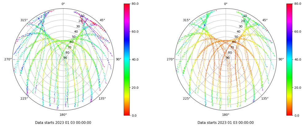
Skyplot for station TALV. Parameter M1C Data file TALV00ESP_R_2023003.xtr Skyplot for station TALV. Parameter M2P Data file TALV00ESP_R_2023003.xtr
