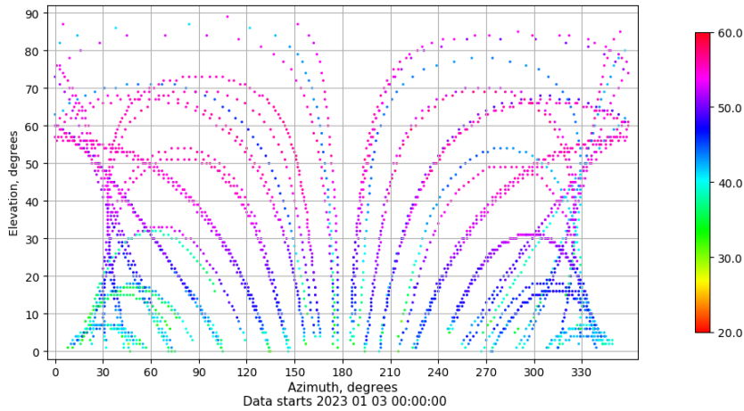
Azimuth-elevation plot for station TALV. Signal to Noise S1C Data file TALV00ESP_R_2023003.xtr
