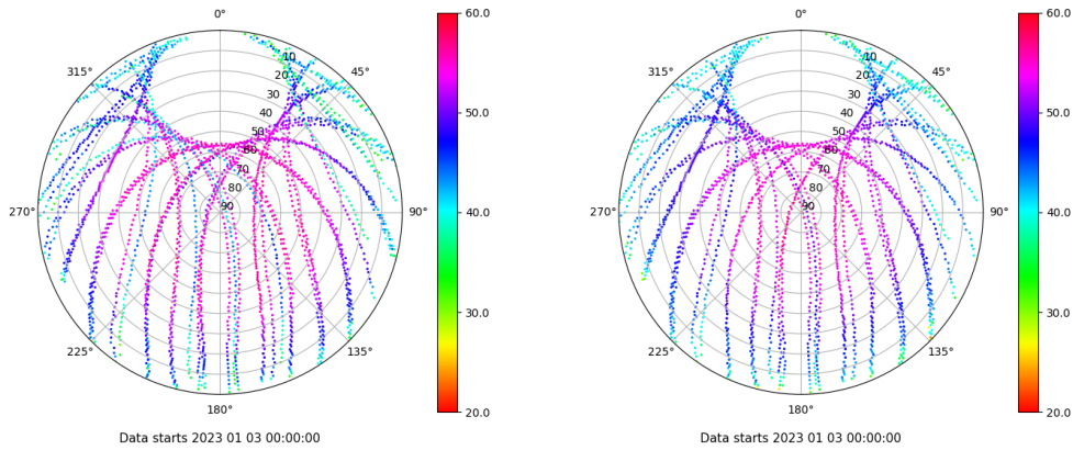
Skyplot for station TALV. Signal to Noise S1C Data file TALV00ESP_R_2023003.xtr Skyplot for station TALV. Signal to Noise S2P Data file TALV00ESP_R_2023003.xtr
