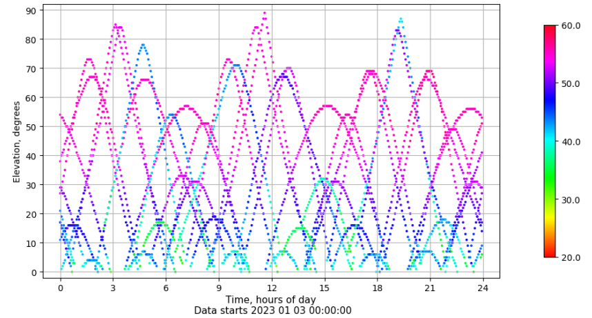
Time-elevation plot for station TALV. Signal to Noise S1C Data file TALV00ESP_R_2023003.xtr
