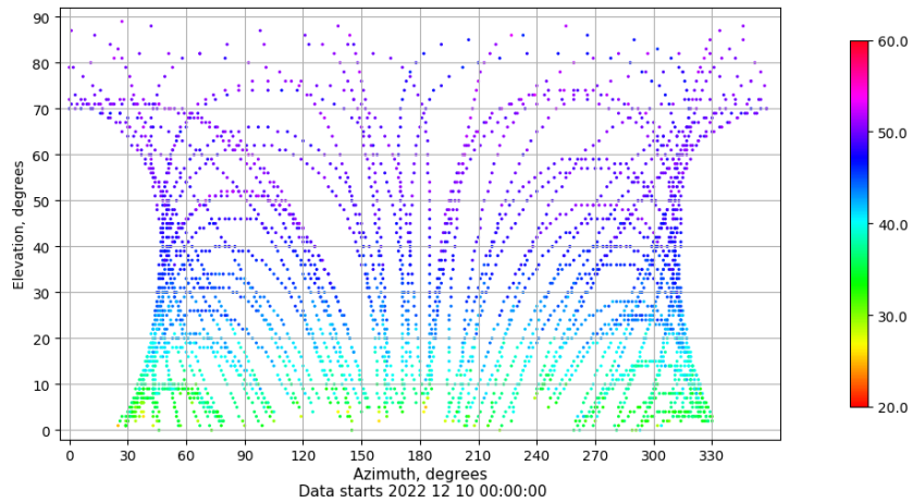
Azimuth-elevation plot for station TALV. Signal to Noise S1C Data file TALV00ESP_R_2022344.xtr
