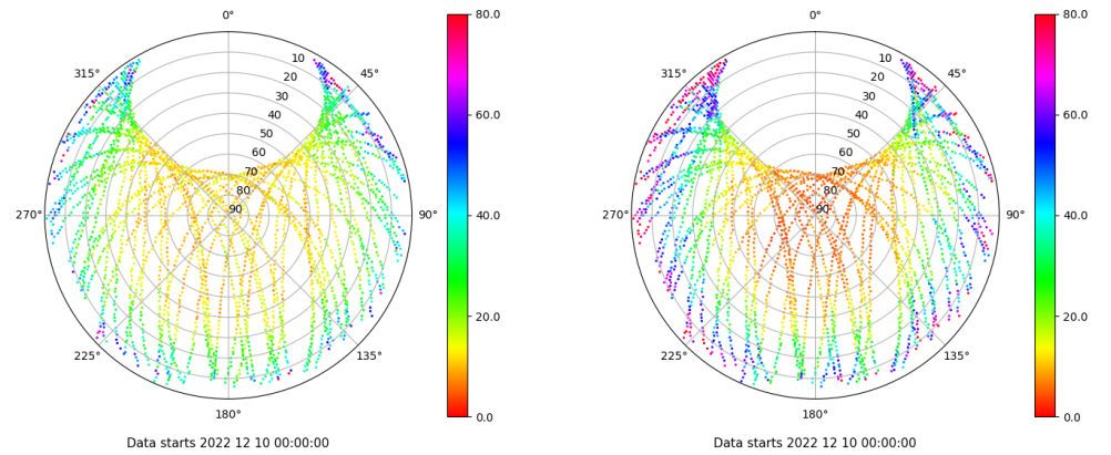
Skyplot for station TALV. Parameter M1C Data file TALV00ESP_R_2022344.xtr Skyplot for station TALV. Parameter M2W Data file TALV00ESP_R_2022344.xtr
