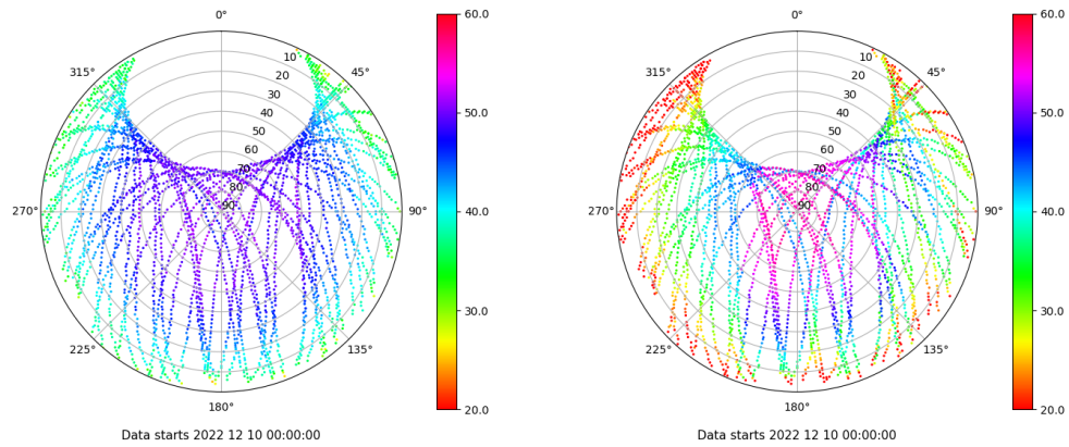
Skyplot for station TALV. Signal to Noise S1C Data file TALV00ESP_R_2022344.xtr Skyplot for station TALV. Signal to Noise S2W Data file TALV00ESP_R_2022344.xtr
