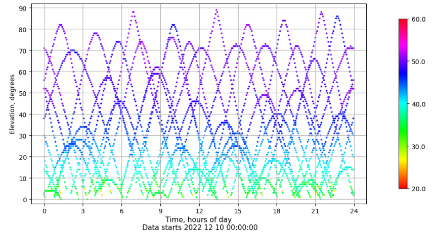
Time-elevation plot for station TALV. Signal to Noise S1C Data file TALV00ESP_R_2022344.xtr
