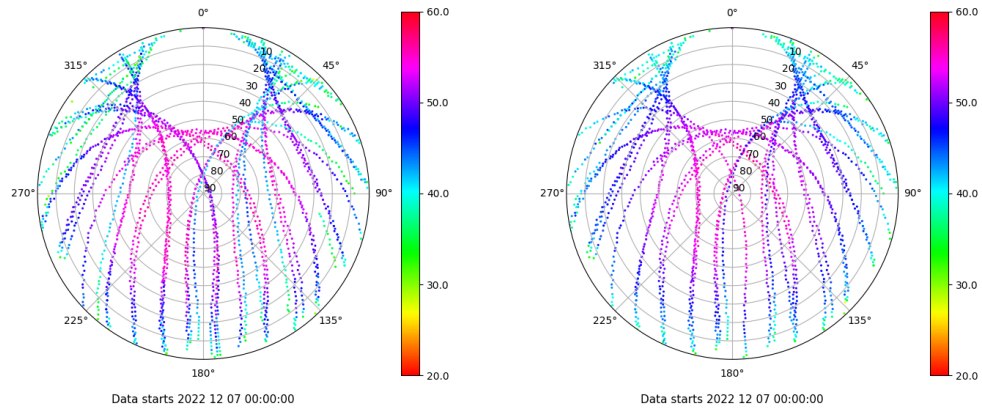
Skyplot for station TALV. Signal to Noise S1C Data file TALV00ESP_R_2022341.xtr Skyplot for station TALV. Signal to Noise S2P Data file TALV00ESP_R_2022341.xtr
