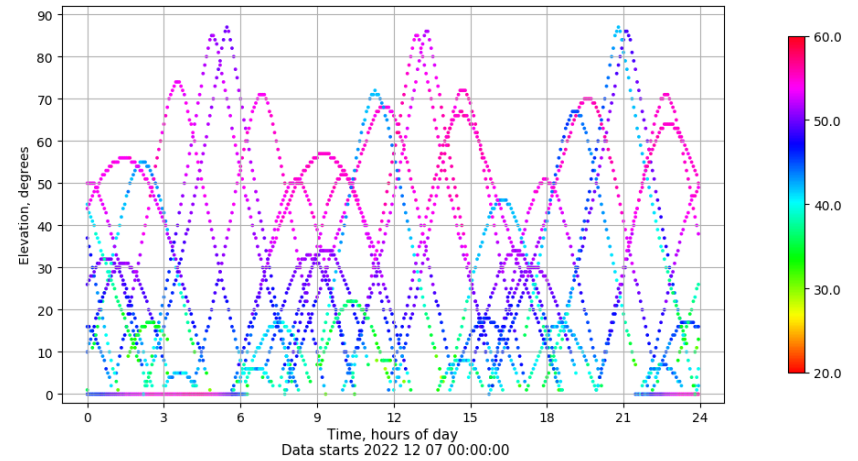
Time-elevation plot for station TALV. Signal to Noise S1C Data file TALV00ESP_R_2022341.xtr
