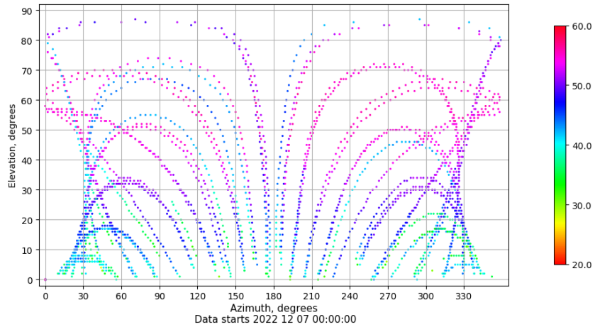
Azimuth-elevation plot for station TALV. Signal to Noise S1C Data file TALV00ESP_R_2022341.xtr
