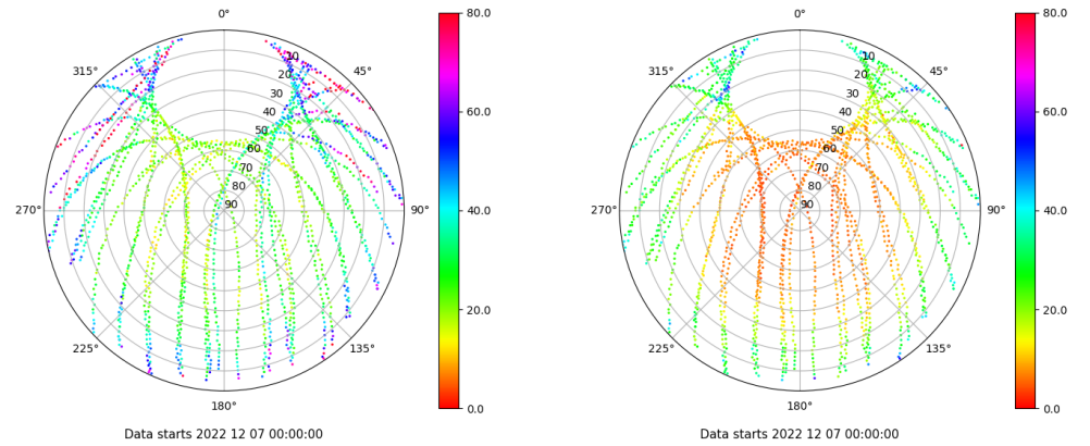
Skyplot for station TALV. Parameter M1C Data file TALV00ESP_R_2022341.xtr Skyplot for station TALV. Parameter M2P Data file TALV00ESP_R_2022341.xtr
