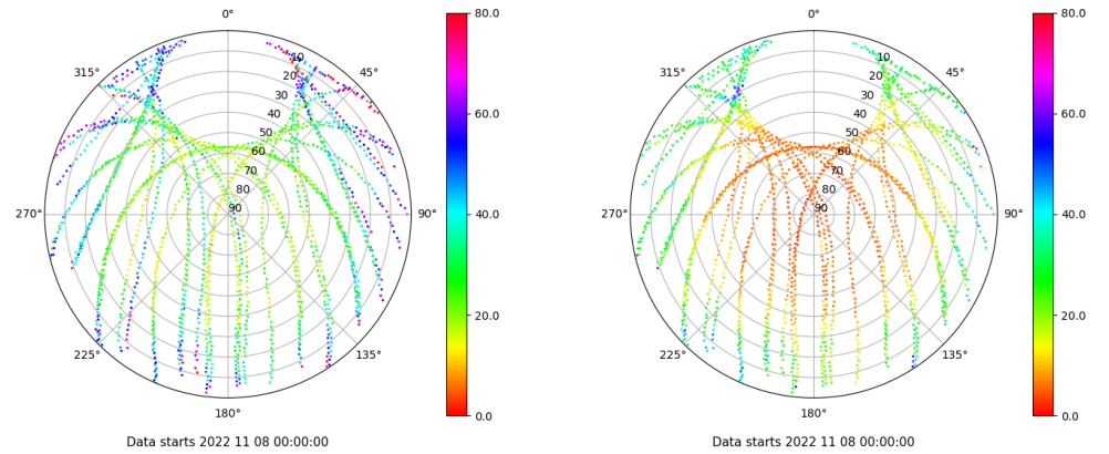
Skyplot for station TALV. Parameter M1C Data file TALV00ESP_R_2022312.xtr Skyplot for station TALV. Parameter M2P Data file TALV00ESP_R_2022312.xtr
