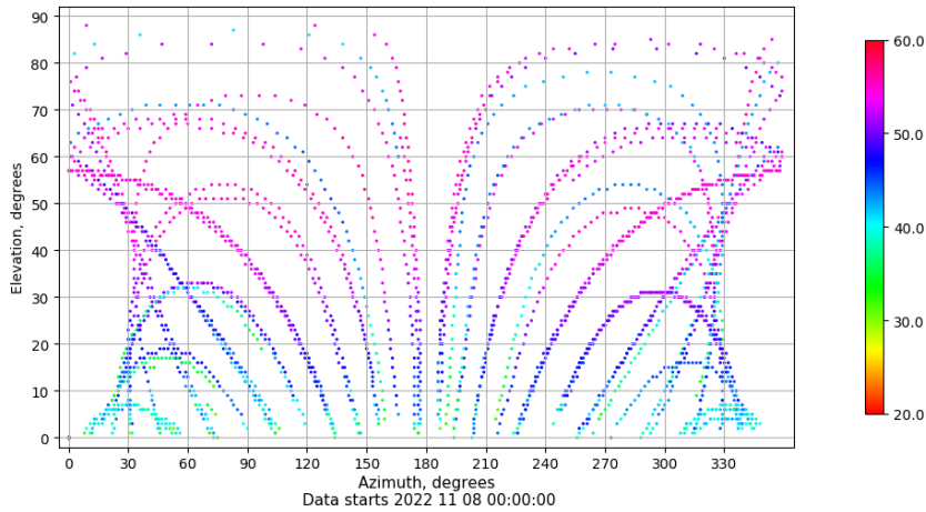
Azimuth-elevation plot for station TALV. Signal to Noise S1C Data file TALV00ESP_R_2022312.xtr
