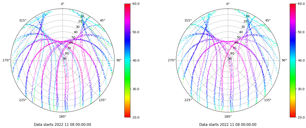
Skyplot for station TALV. Signal to Noise S1C Data file TALV00ESP_R_2022312.xtr Skyplot for station TALV. Signal to Noise S2P Data file TALV00ESP_R_2022312.xtr
