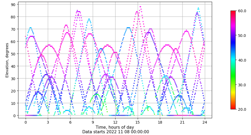
Time-elevation plot for station TALV. Signal to Noise S1C Data file TALV00ESP_R_2022312.xtr
