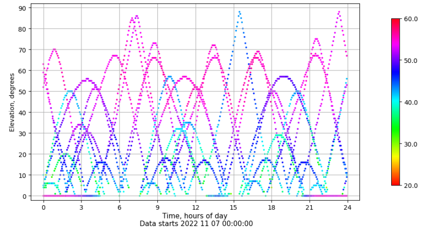
Time-elevation plot for station TALV. Signal to Noise S1C Data file TALV00ESP_R_2022311.xtr
