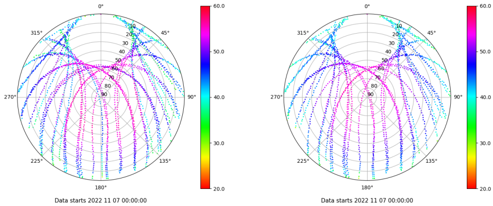
Skyplot for station TALV. Signal to Noise S1C Data file TALV00ESP_R_2022311.xtr Skyplot for station TALV. Signal to Noise S2P Data file TALV00ESP_R_2022311.xtr
