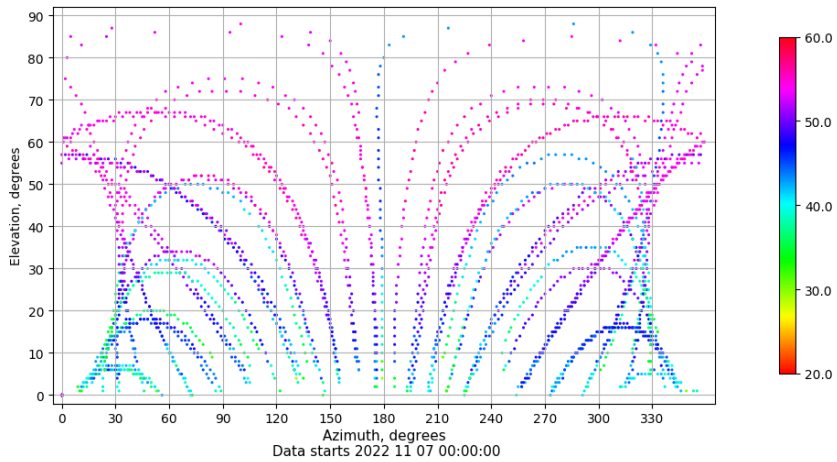
Azimuth-elevation plot for station TALV. Signal to Noise S1C Data file TALV00ESP_R_2022311.xtr
