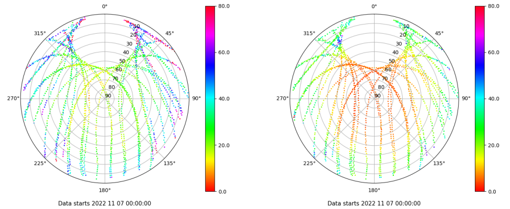
Skyplot for station TALV. Parameter M1C Data file TALV00ESP_R_2022311.xtr Skyplot for station TALV. Parameter M2P Data file TALV00ESP_R_2022311.xtr
