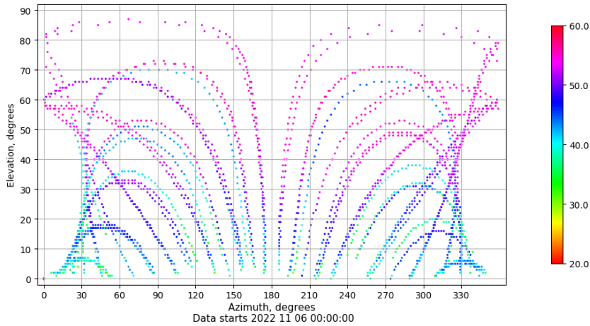
Azimuth-elevation plot for station TALV. Signal to Noise S1C Data file TALV00ESP_R_2022310.xtr
