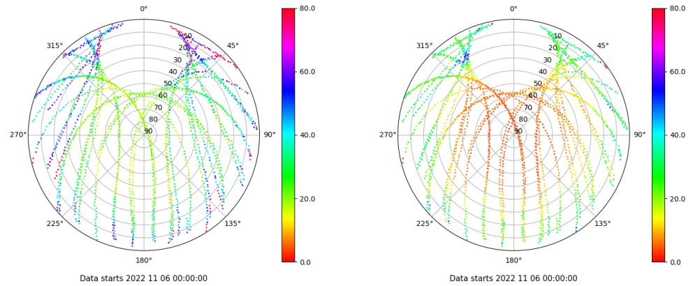
Skyplot for station TALV. Parameter M1C Data file TALV00ESP_R_2022310.xtr Skyplot for station TALV. Parameter M2P Data file TALV00ESP_R_2022310.xtr
