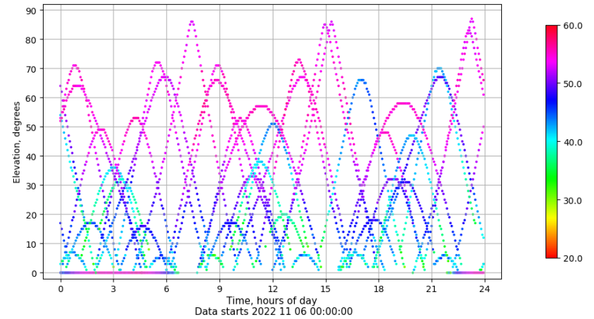
Time-elevation plot for station TALV. Signal to Noise S1C Data file TALV00ESP_R_2022310.xtr
