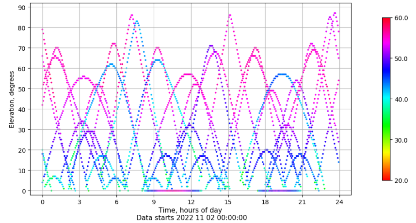
Time-elevation plot for station TALV. Signal to Noise S1C Data file TALV00ESP_R_2022306.xtr
