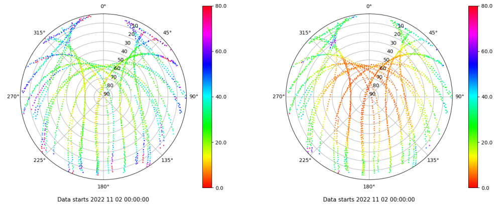
Skyplot for station TALV. Parameter M1C Data file TALV00ESP_R_2022306.xtr Skyplot for station TALV. Parameter M2P Data file TALV00ESP_R_2022306.xtr
