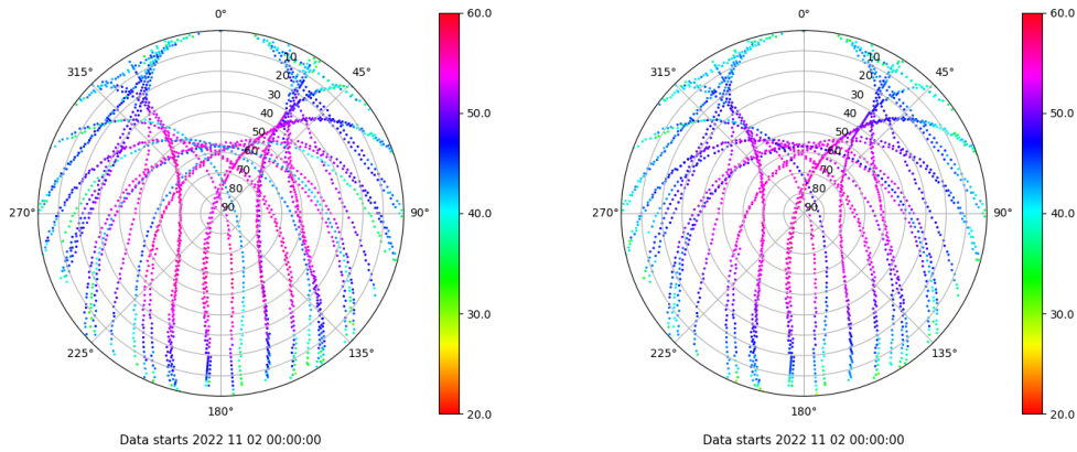
Skyplot for station TALV. Signal to Noise S1C Data file TALV00ESP_R_2022306.xtr Skyplot for station TALV. Signal to Noise S2P Data file TALV00ESP_R_2022306.xtr
