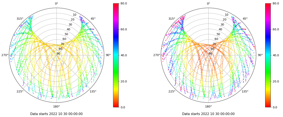
Skyplot for station TALV. Parameter M1C Data file TALV00ESP_R_2022303.xtr Skyplot for station TALV. Parameter M2W Data file TALV00ESP_R_2022303.xtr
