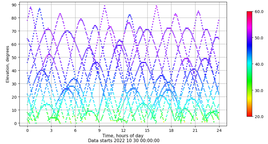
Time-elevation plot for station TALV. Signal to Noise S1C Data file TALV00ESP_R_2022303.xtr
