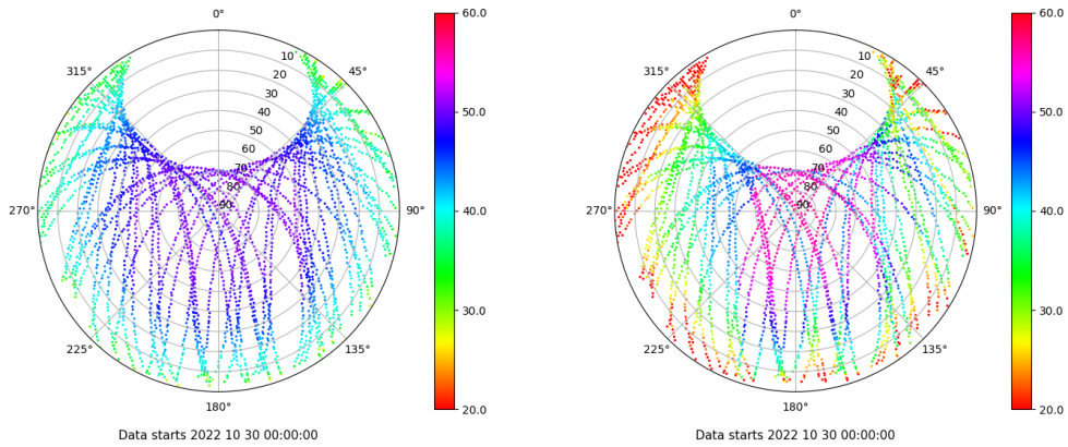
Skyplot for station TALV. Signal to Noise S1C Data file TALV00ESP_R_2022303.xtr Skyplot for station TALV. Signal to Noise S2W Data file TALV00ESP_R_2022303.xtr
