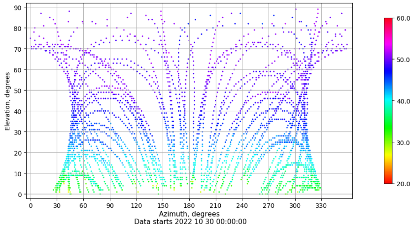
Azimuth-elevation plot for station TALV. Signal to Noise S1C Data file TALV00ESP_R_2022303.xtr
