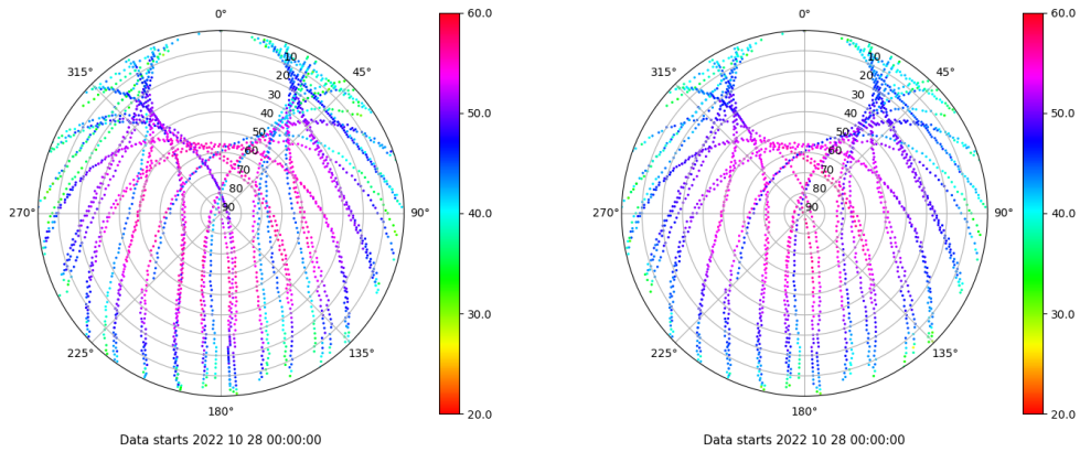
Skyplot for station TALV. Signal to Noise S1C Data file TALV00ESP_R_2022301.xtr Skyplot for station TALV. Signal to Noise S2P Data file TALV00ESP_R_2022301.xtr
