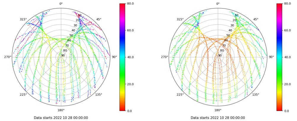
Skyplot for station TALV. Parameter M1C Data file TALV00ESP_R_2022301.xtr Skyplot for station TALV. Parameter M2P Data file TALV00ESP_R_2022301.xtr
