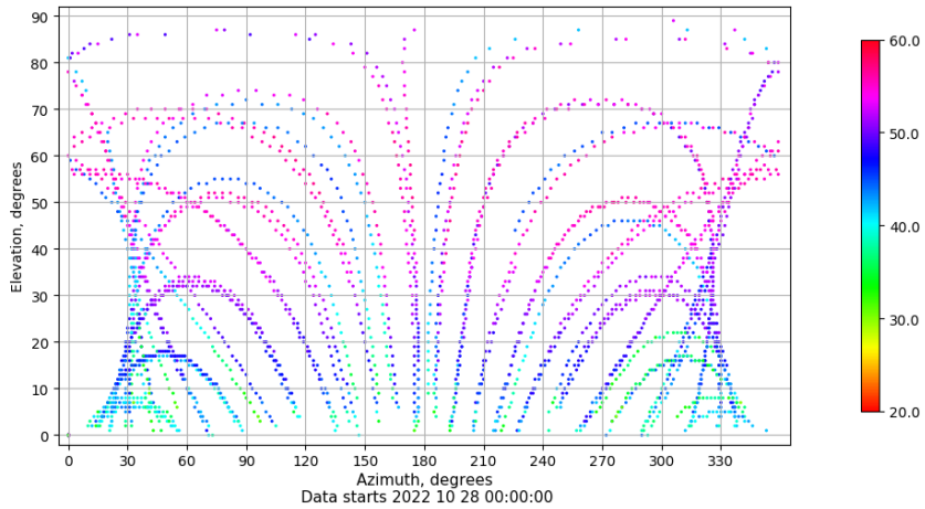
Azimuth-elevation plot for station TALV. Signal to Noise S1C Data file TALV00ESP_R_2022301.xtr
