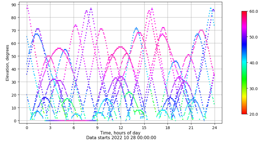
Time-elevation plot for station TALV. Signal to Noise S1C Data file TALV00ESP_R_2022301.xtr
