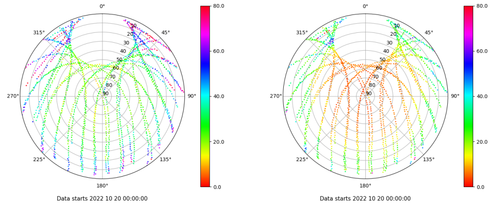
Skyplot for station TALV. Parameter M1C Data file TALV00ESP_R_2022293.xtr Skyplot for station TALV. Parameter M2P Data file TALV00ESP_R_2022293.xtr
