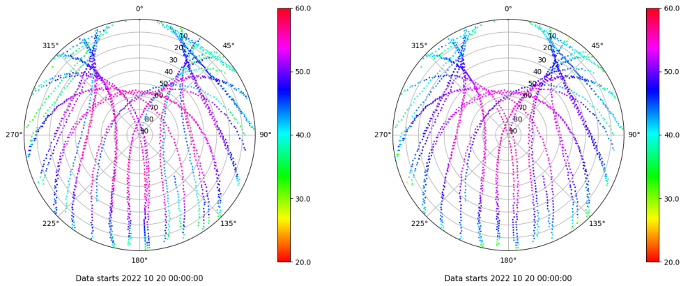
Skyplot for station TALV. Signal to Noise S1C Data file TALV00ESP_R_2022293.xtr Skyplot for station TALV. Signal to Noise S2P Data file TALV00ESP_R_2022293.xtr
