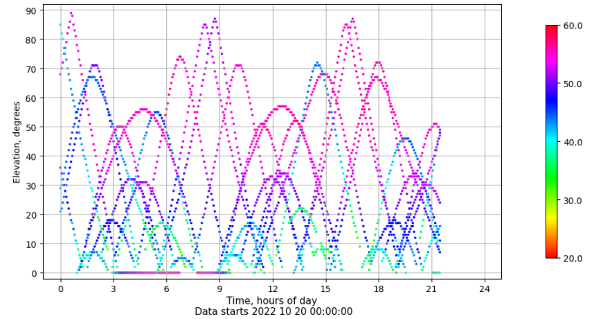
Time-elevation plot for station TALV. Signal to Noise S1C Data file TALV00ESP_R_2022293.xtr
