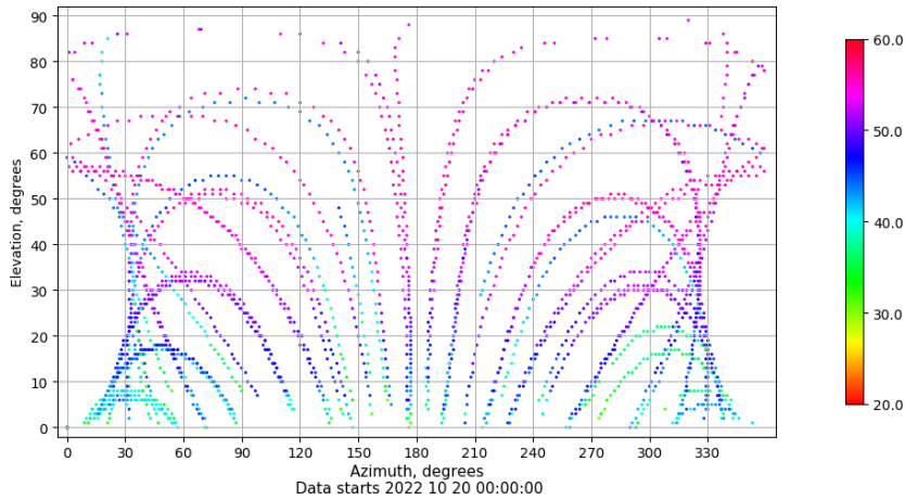
Azimuth-elevation plot for station TALV. Signal to Noise S1C Data file TALV00ESP_R_2022293.xtr
