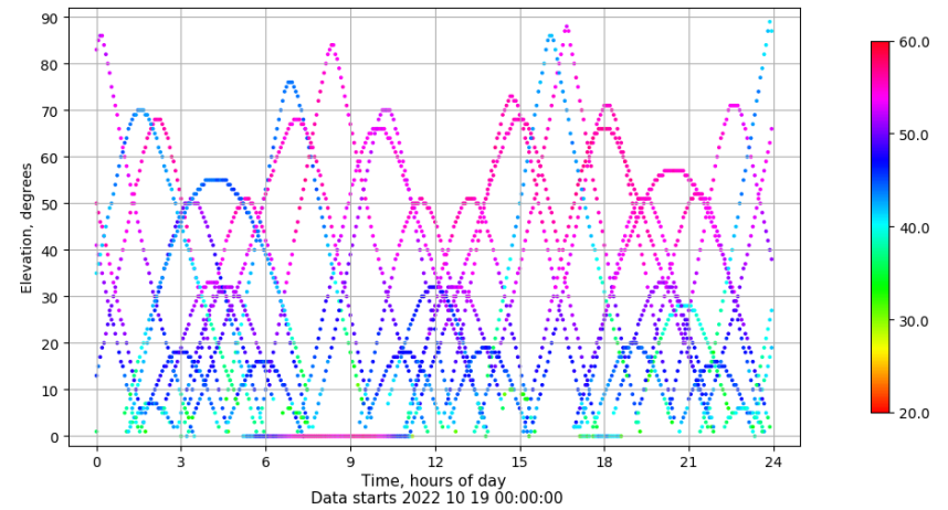
Time-elevation plot for station TALV. Signal to Noise S1C Data file TALV00ESP_R_2022292.xtr
