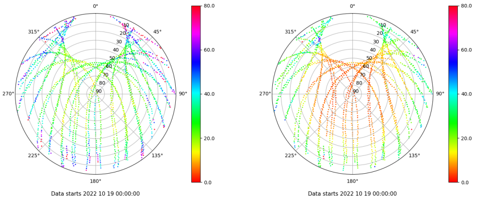
Skyplot for station TALV. Parameter M1C Data file TALV00ESP_R_2022292.xtr Skyplot for station TALV. Parameter M2P Data file TALV00ESP_R_2022292.xtr
