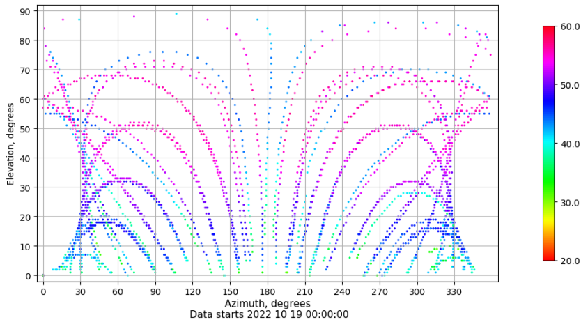
Azimuth-elevation plot for station TALV. Signal to Noise S1C Data file TALV00ESP_R_2022292.xtr
