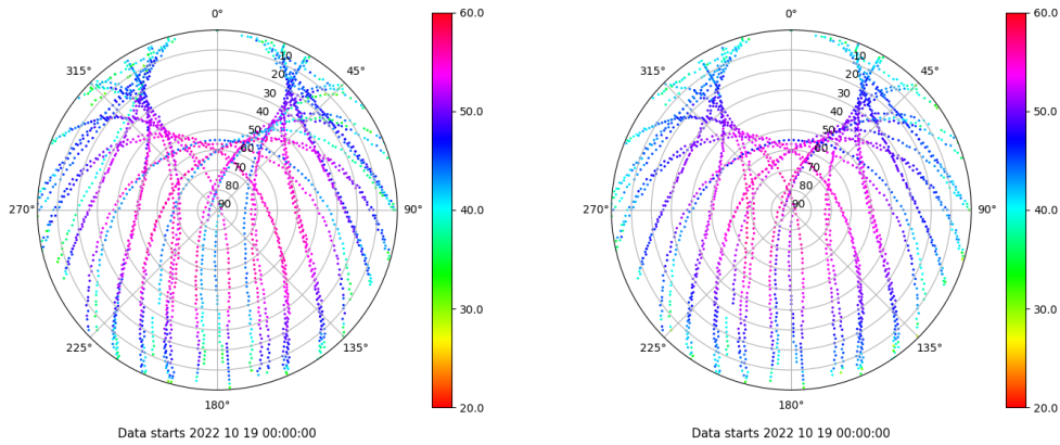
Skyplot for station TALV. Signal to Noise S1C Data file TALV00ESP_R_2022292.xtr Skyplot for station TALV. Signal to Noise S2P Data file TALV00ESP_R_2022292.xtr
