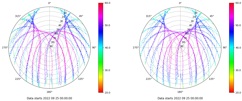
Skyplot for station TALV. Signal to Noise S1C Data file TALV00ESP_R_2022268.xtr Skyplot for station TALV. Signal to Noise S2P Data file TALV00ESP_R_2022268.xtr
