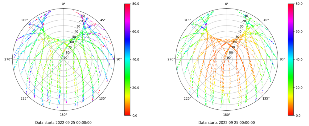
Skyplot for station TALV. Parameter M1C Data file TALV00ESP_R_2022268.xtr Skyplot for station TALV. Parameter M2P Data file TALV00ESP_R_2022268.xtr
