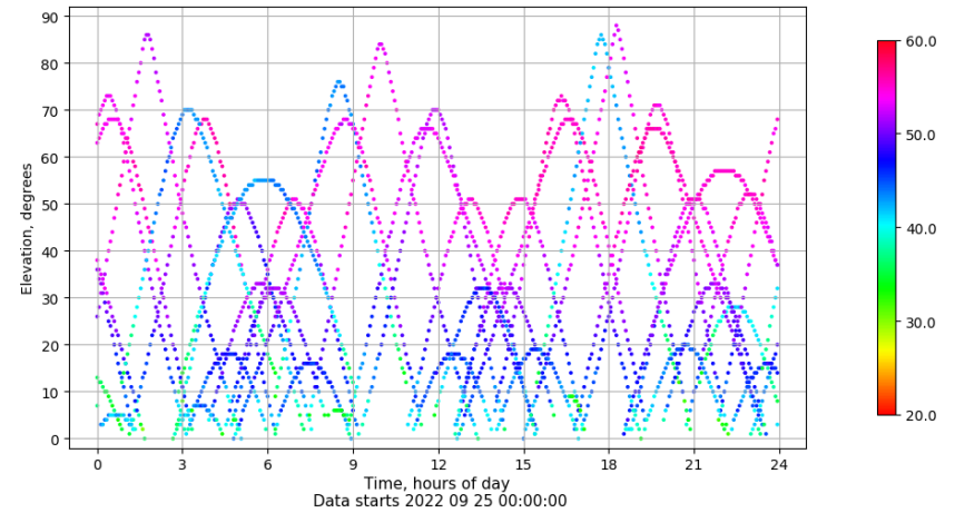
Time-elevation plot for station TALV. Signal to Noise S1C Data file TALV00ESP_R_2022268.xtr
