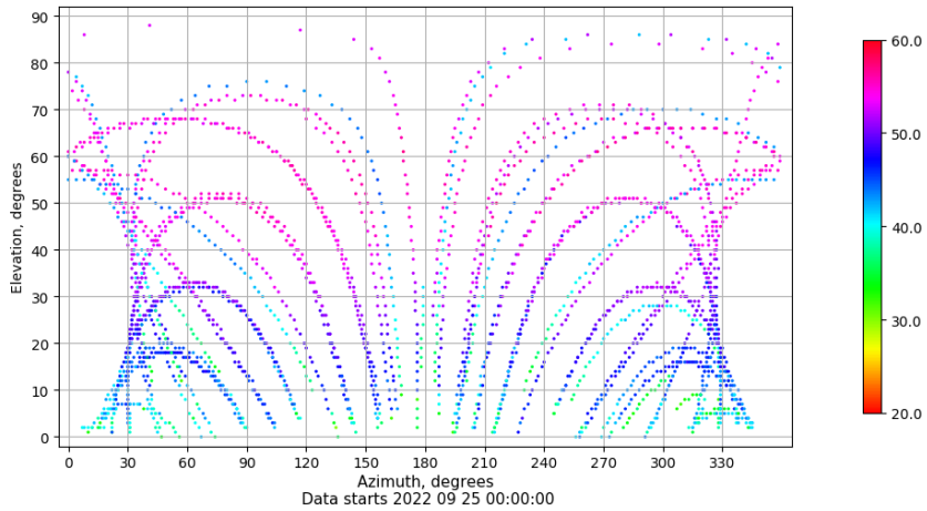
Azimuth-elevation plot for station TALV. Signal to Noise S1C Data file TALV00ESP_R_2022268.xtr
