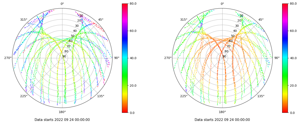
Skyplot for station TALV. Parameter M1C Data file TALV00ESP_R_2022267.xtr Skyplot for station TALV. Parameter M2P Data file TALV00ESP_R_2022267.xtr
