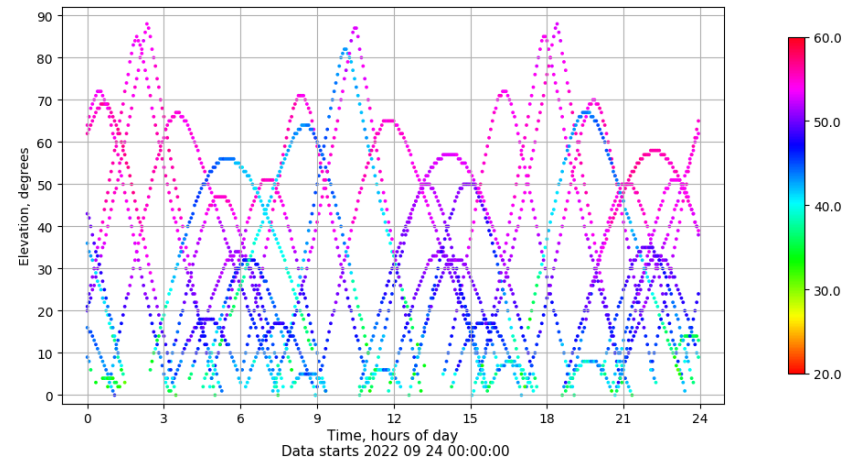
Time-elevation plot for station TALV. Signal to Noise S1C Data file TALV00ESP_R_2022267.xtr
