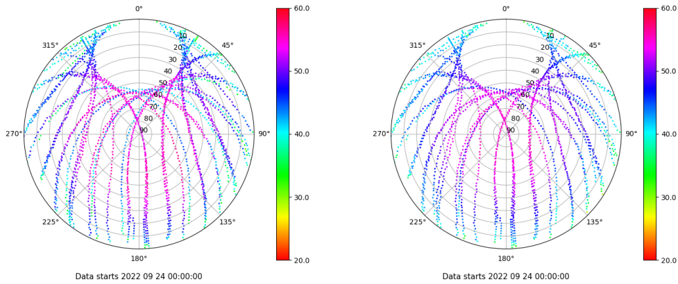
Skyplot for station TALV. Signal to Noise S1C Data file TALV00ESP_R_2022267.xtr Skyplot for station TALV. Signal to Noise S2P Data file TALV00ESP_R_2022267.xtr
