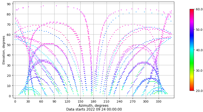
Azimuth-elevation plot for station TALV. Signal to Noise S1C Data file TALV00ESP_R_2022267.xtr
