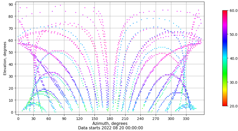
Azimuth-elevation plot for station TALV. Signal to Noise S1C Data file TALV00ESP_R_2022232.xtr
