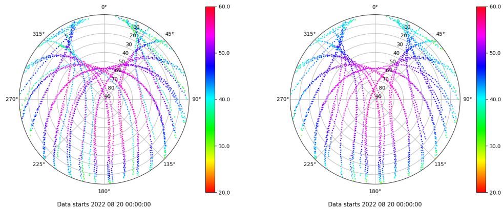
Skyplot for station TALV. Signal to Noise S1C Data file TALV00ESP_R_2022232.xtr Skyplot for station TALV. Signal to Noise S2P Data file TALV00ESP_R_2022232.xtr
