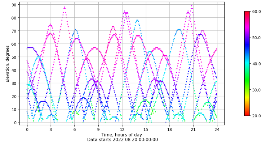
Time-elevation plot for station TALV. Signal to Noise S1C Data file TALV00ESP_R_2022232.xtr
