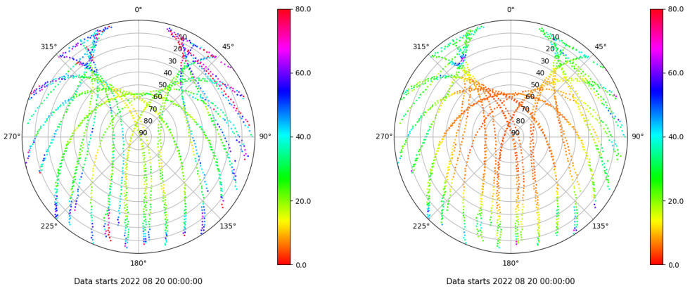
Skyplot for station TALV. Parameter M1C Data file TALV00ESP_R_2022232.xtr Skyplot for station TALV. Parameter M2P Data file TALV00ESP_R_2022232.xtr
