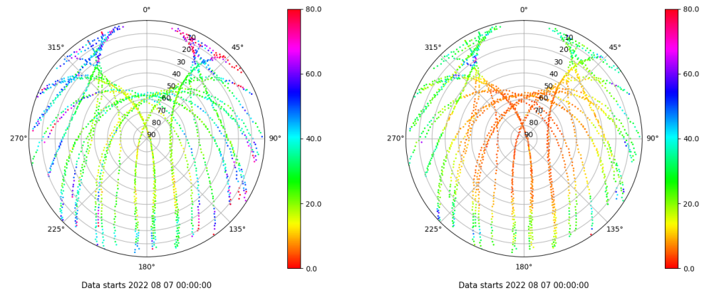
Skyplot for station TALV. Parameter M1C Data file TALV00ESP_R_2022219.xtr Skyplot for station TALV. Parameter M2P Data file TALV00ESP_R_2022219.xtr
