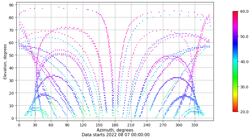
Azimuth-elevation plot for station TALV. Signal to Noise S1C Data file TALV00ESP_R_2022219.xtr
