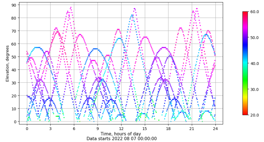
Time-elevation plot for station TALV. Signal to Noise S1C Data file TALV00ESP_R_2022219.xtr
