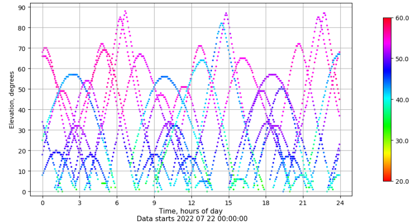
Time-elevation plot for station TALV. Signal to Noise S1C Data file TALV00ESP_R_2022203.xtr
