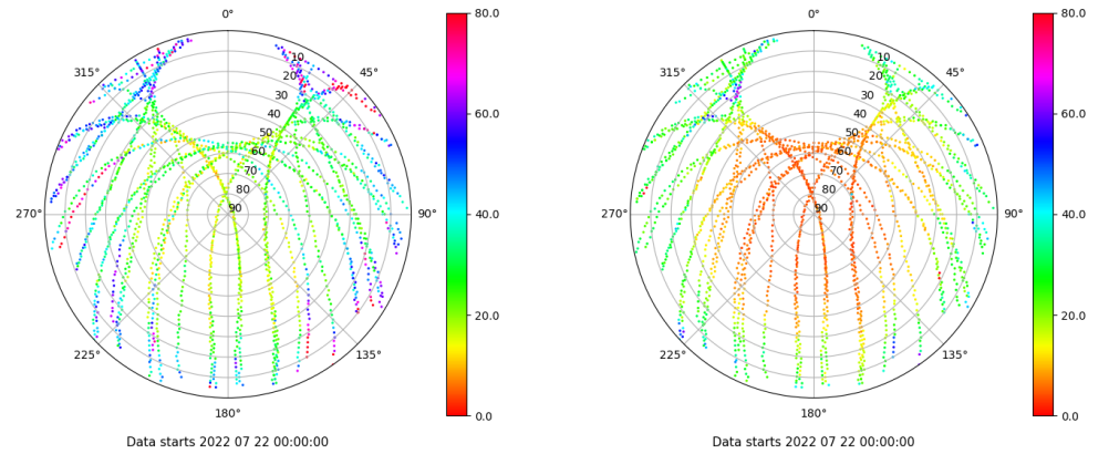
Skyplot for station TALV. Parameter M1C Data file TALV00ESP_R_2022203.xtr Skyplot for station TALV. Parameter M2P Data file TALV00ESP_R_2022203.xtr
