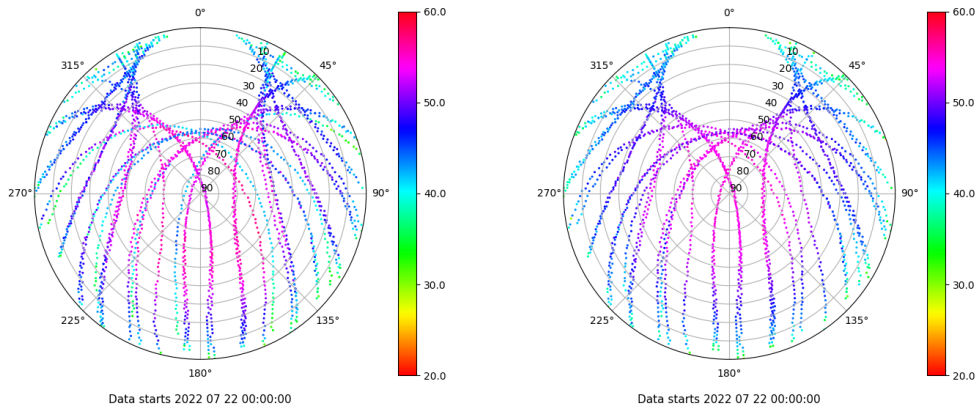
Skyplot for station TALV. Signal to Noise S1C Data file TALV00ESP_R_2022203.xtr Skyplot for station TALV. Signal to Noise S2P Data file TALV00ESP_R_2022203.xtr
