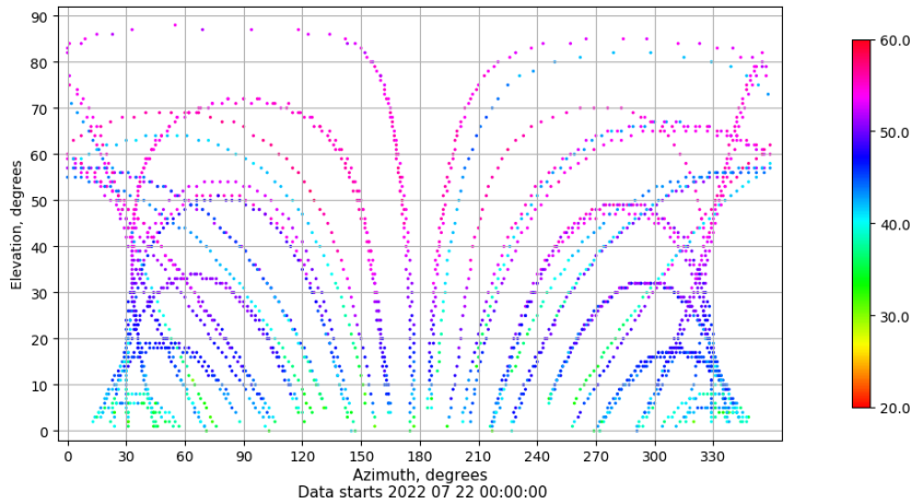
Azimuth-elevation plot for station TALV. Signal to Noise S1C Data file TALV00ESP_R_2022203.xtr
