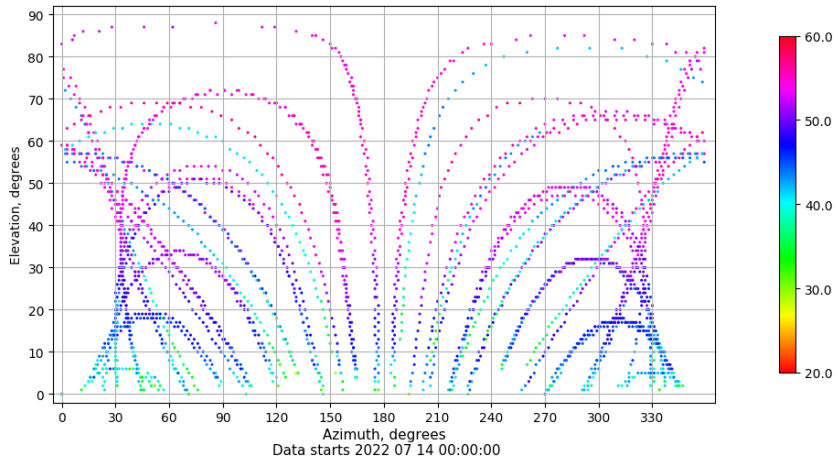
Azimuth-elevation plot for station TALV. Signal to Noise S1C Data file TALV00ESP_R_2022195.xtr
