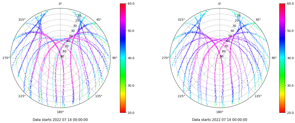
Skyplot for station TALV. Signal to Noise S1C Data file TALV00ESP_R_2022195.xtr Skyplot for station TALV. Signal to Noise S2P Data file TALV00ESP_R_2022195.xtr
