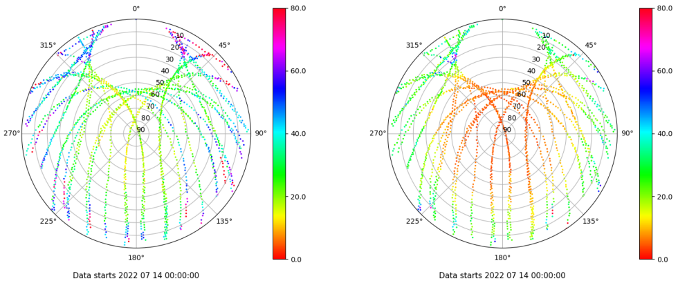
Skyplot for station TALV. Parameter M1C Data file TALV00ESP_R_2022195.xtr Skyplot for station TALV. Parameter M2P Data file TALV00ESP_R_2022195.xtr
