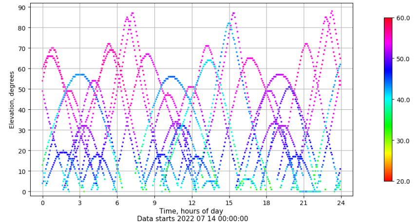
Time-elevation plot for station TALV. Signal to Noise S1C Data file TALV00ESP_R_2022195.xtr
