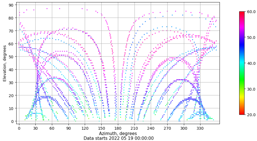
Azimuth-elevation plot for station TALV. Signal to Noise S1C Data file TALV00ESP_R_2022139.xtr
