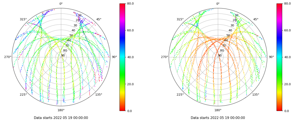
Skyplot for station TALV. Parameter M1C Data file TALV00ESP_R_2022139.xtr Skyplot for station TALV. Parameter M2P Data file TALV00ESP_R_2022139.xtr
