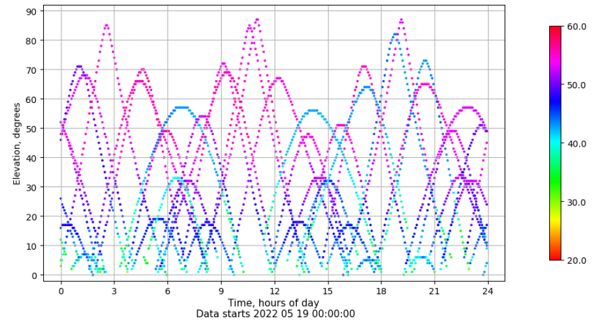
Time-elevation plot for station TALV. Signal to Noise S1C Data file TALV00ESP_R_2022139.xtr
