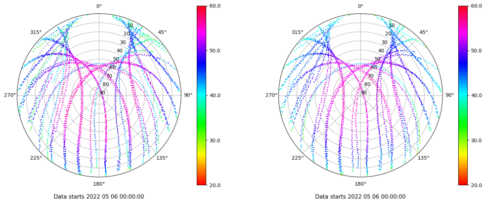
Skyplot for station TALV. Signal to Noise S1C Data file TALV00ESP_R_2022126.xtr Skyplot for station TALV. Signal to Noise S2P Data file TALV00ESP_R_2022126.xtr
