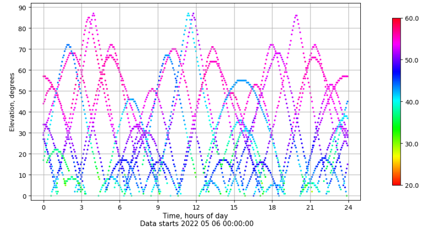
Time-elevation plot for station TALV. Signal to Noise S1C Data file TALV00ESP_R_2022126.xtr
