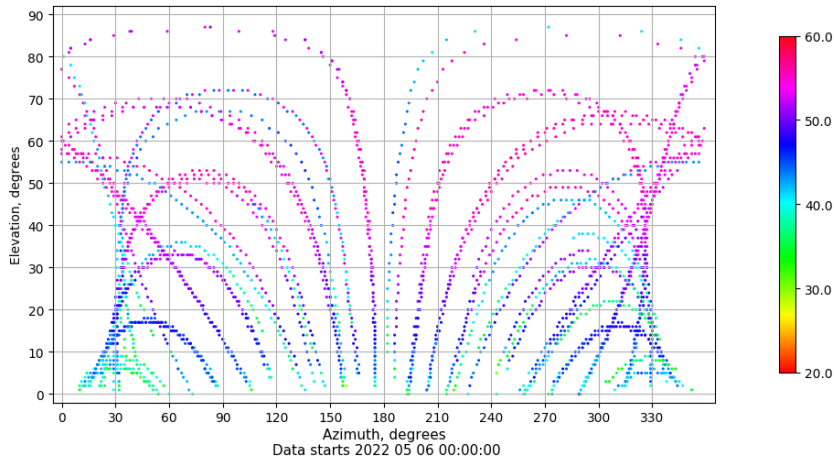
Azimuth-elevation plot for station TALV. Signal to Noise S1C Data file TALV00ESP_R_2022126.xtr
