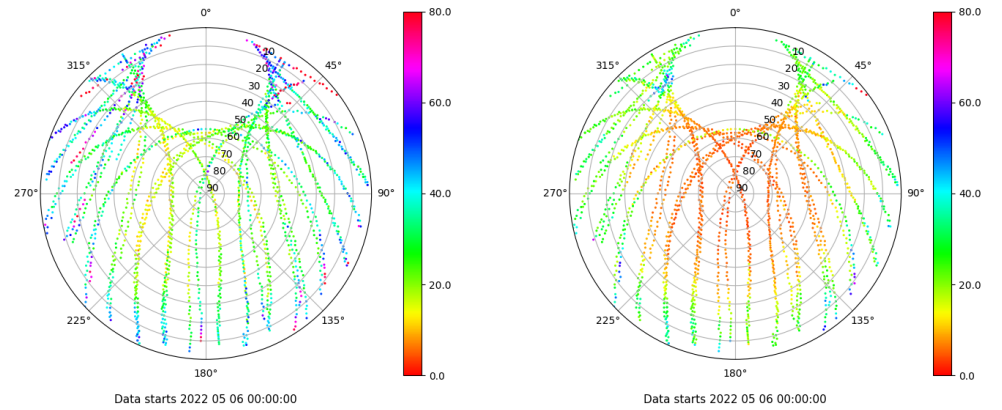
Skyplot for station TALV. Parameter M1C Data file TALV00ESP_R_2022126.xtr Skyplot for station TALV. Parameter M2P Data file TALV00ESP_R_2022126.xtr
