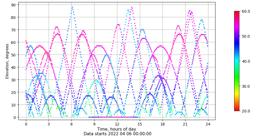
Time-elevation plot for station TALV. Signal to Noise S1C Data file TALV00ESP_R_2022096.xtr
