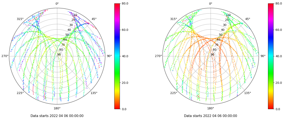
Skyplot for station TALV. Parameter M1C Data file TALV00ESP_R_2022096.xtr Skyplot for station TALV. Parameter M2P Data file TALV00ESP_R_2022096.xtr
