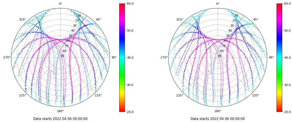
Skyplot for station TALV. Signal to Noise S1C Data file TALV00ESP_R_2022096.xtr Skyplot for station TALV. Signal to Noise S2P Data file TALV00ESP_R_2022096.xtr
