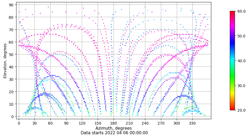
Azimuth-elevation plot for station TALV. Signal to Noise S1C Data file TALV00ESP_R_2022096.xtr
