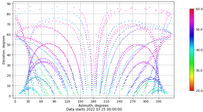
Azimuth-elevation plot for station TALV. Signal to Noise S1C Data file TALV00ESP_R_2022084.xtr
