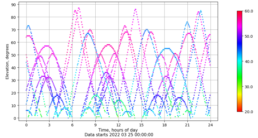
Time-elevation plot for station TALV. Signal to Noise S1C Data file TALV00ESP_R_2022084.xtr
