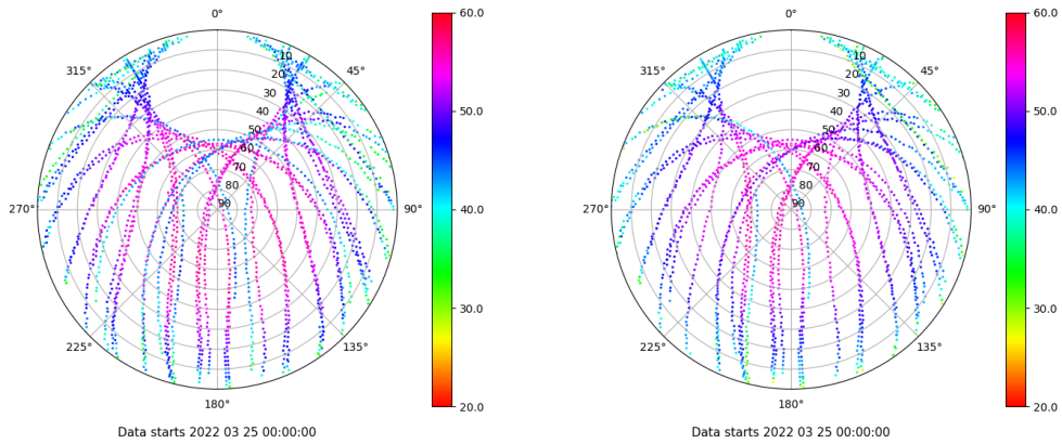
Skyplot for station TALV. Signal to Noise S1C Data file TALV00ESP_R_2022084.xtr Skyplot for station TALV. Signal to Noise S2P Data file TALV00ESP_R_2022084.xtr
