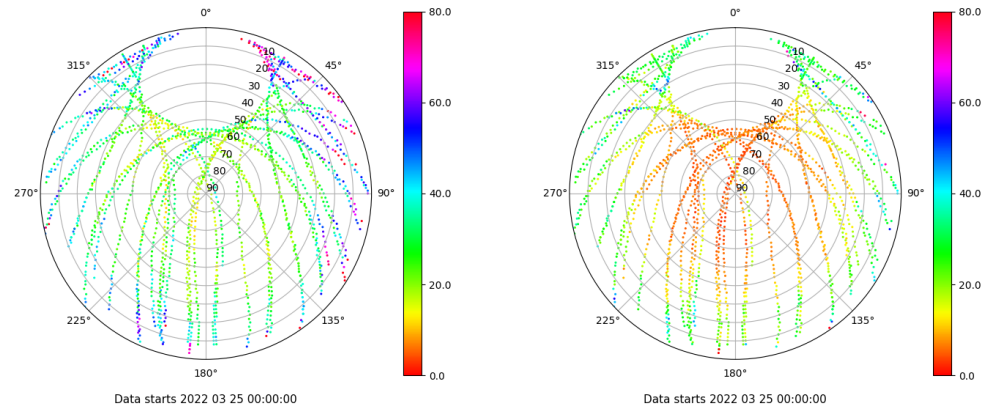
Skyplot for station TALV. Parameter M1C Data file TALV00ESP_R_2022084.xtr Skyplot for station TALV. Parameter M2P Data file TALV00ESP_R_2022084.xtr
