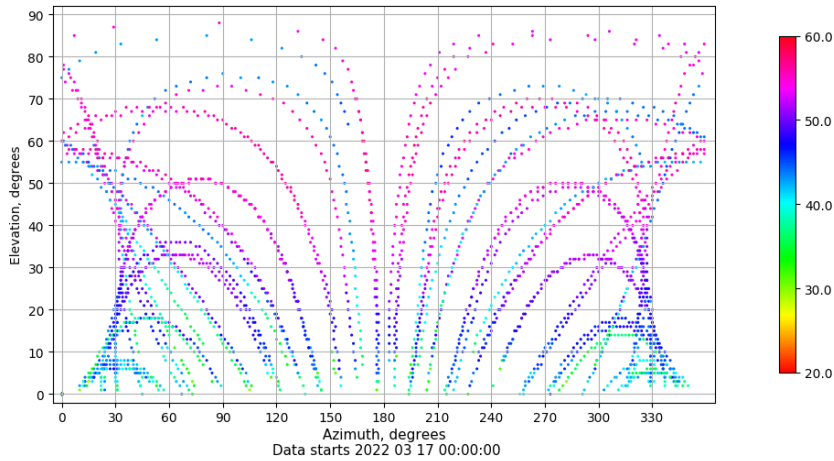
Azimuth-elevation plot for station TALV. Signal to Noise S1C Data file TALV00ESP_R_2022076.xtr
