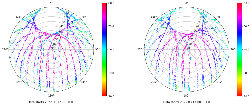
Skyplot for station TALV. Signal to Noise S1C Data file TALV00ESP_R_2022076.xtr Skyplot for station TALV. Signal to Noise S2P Data file TALV00ESP_R_2022076.xtr
