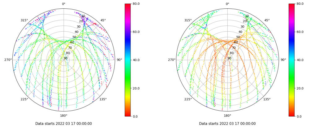
Skyplot for station TALV. Parameter M1C Data file TALV00ESP_R_2022076.xtr Skyplot for station TALV. Parameter M2P Data file TALV00ESP_R_2022076.xtr
