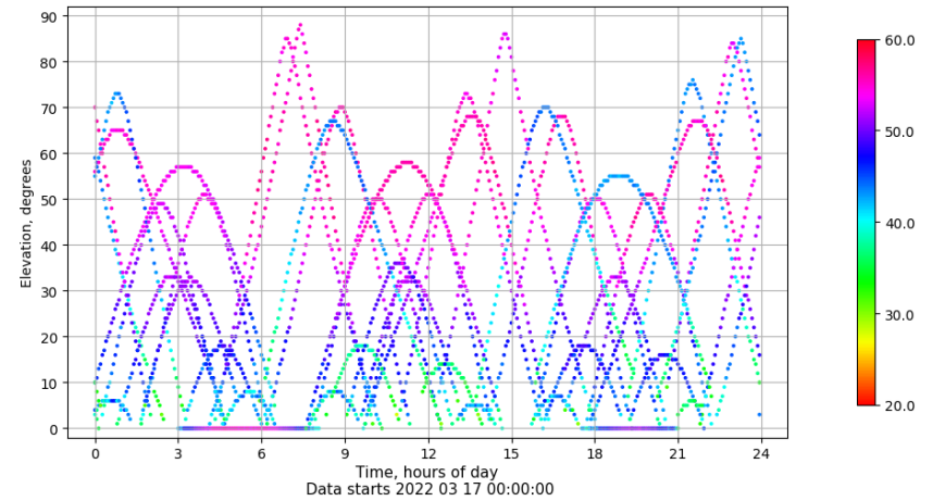
Time-elevation plot for station TALV. Signal to Noise S1C Data file TALV00ESP_R_2022076.xtr
