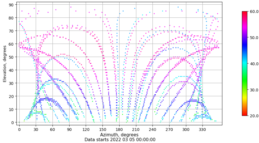
Azimuth-elevation plot for station TALV. Signal to Noise S1C Data file TALV00ESP_R_2022064.xtr
