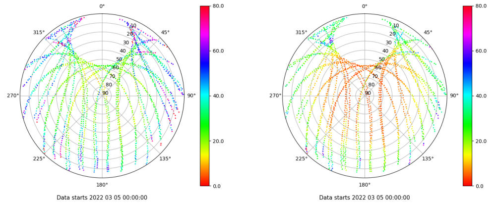
Skyplot for station TALV. Parameter M1C Data file TALV00ESP_R_2022064.xtr Skyplot for station TALV. Parameter M2P Data file TALV00ESP_R_2022064.xtr
