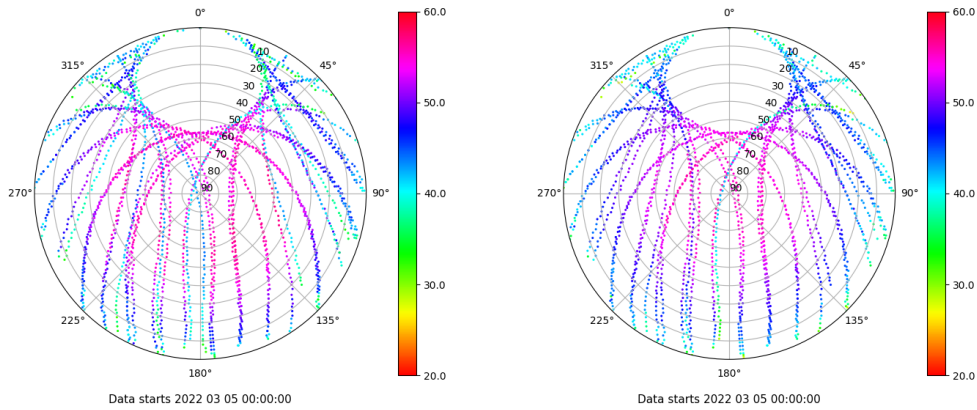
Skyplot for station TALV. Signal to Noise S1C Data file TALV00ESP_R_2022064.xtr Skyplot for station TALV. Signal to Noise S2P Data file TALV00ESP_R_2022064.xtr
