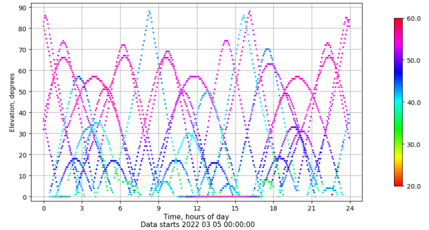
Time-elevation plot for station TALV. Signal to Noise S1C Data file TALV00ESP_R_2022064.xtr
