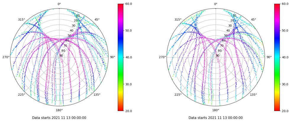
Skyplot for station TALV. Signal to Noise S1C Data file TALV00ESP_R_2021317.xtr Skyplot for station TALV. Signal to Noise S2P Data file TALV00ESP_R_2021317.xtr
