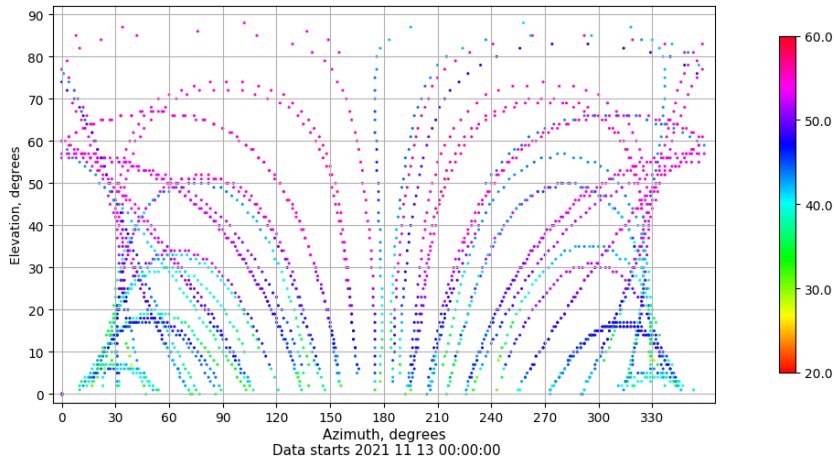
Azimuth-elevation plot for station TALV. Signal to Noise S1C Data file TALV00ESP_R_2021317.xtr
