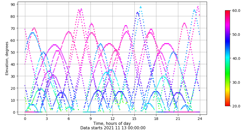
Time-elevation plot for station TALV. Signal to Noise S1C Data file TALV00ESP_R_2021317.xtr
