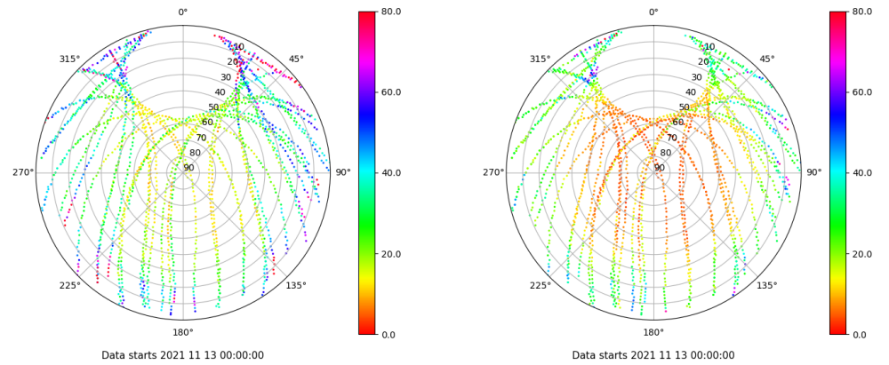
Skyplot for station TALV. Parameter M1C Data file TALV00ESP_R_2021317.xtr Skyplot for station TALV. Parameter M2P Data file TALV00ESP_R_2021317.xtr
