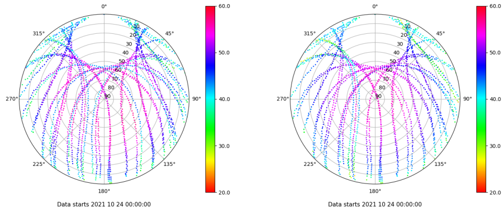
Skyplot for station TALV. Signal to Noise S1C Data file TALV00ESP_R_2021297.xtr Skyplot for station TALV. Signal to Noise S2P Data file TALV00ESP_R_2021297.xtr
