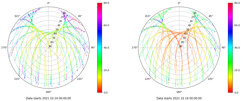
Skyplot for station TALV. Parameter M1C Data file TALV00ESP_R_2021297.xtr Skyplot for station TALV. Parameter M2P Data file TALV00ESP_R_2021297.xtr
