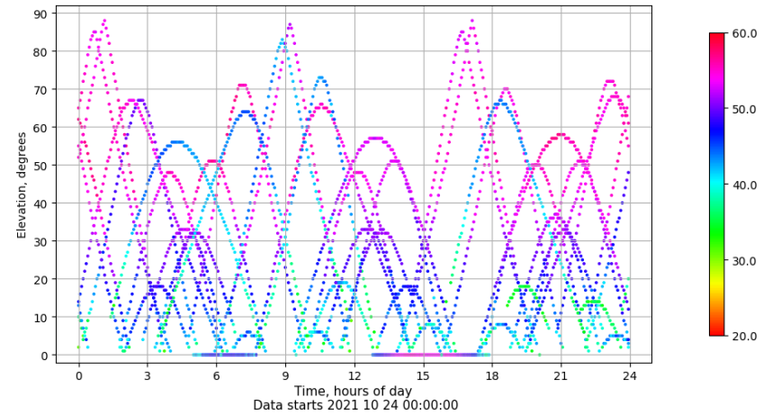
Time-elevation plot for station TALV. Signal to Noise S1C Data file TALV00ESP_R_2021297.xtr
