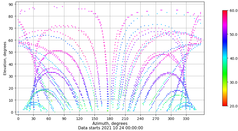
Azimuth-elevation plot for station TALV. Signal to Noise S1C Data file TALV00ESP_R_2021297.xtr
