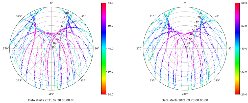
Skyplot for station TALV. Signal to Noise S1C Data file TALV00ESP_R_2021263.xtr Skyplot for station TALV. Signal to Noise S2P Data file TALV00ESP_R_2021263.xtr
