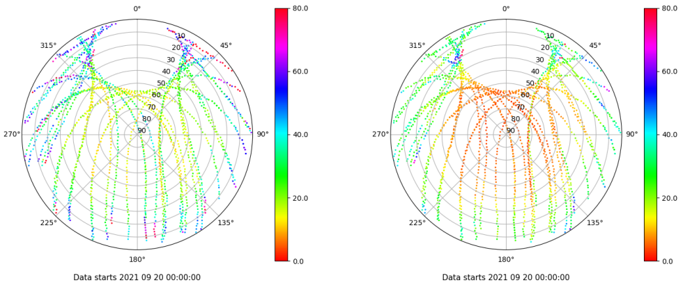
Skyplot for station TALV. Parameter M1C Data file TALV00ESP_R_2021263.xtr Skyplot for station TALV. Parameter M2P Data file TALV00ESP_R_2021263.xtr
