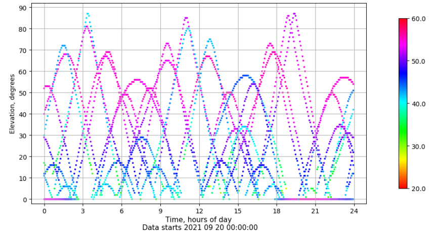
Time-elevation plot for station TALV. Signal to Noise S1C Data file TALV00ESP_R_2021263.xtr
