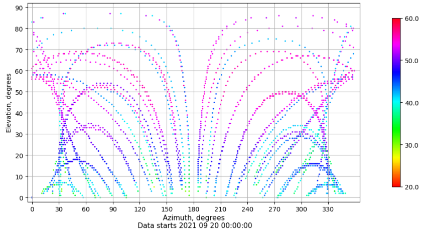
Azimuth-elevation plot for station TALV. Signal to Noise S1C Data file TALV00ESP_R_2021263.xtr
