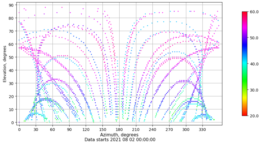
Azimuth-elevation plot for station TALV. Signal to Noise S1C Data file TALV00ESP_R_2021214.xtr
