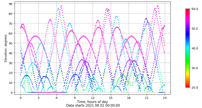
Time-elevation plot for station TALV. Signal to Noise S1C Data file TALV00ESP_R_2021214.xtr
