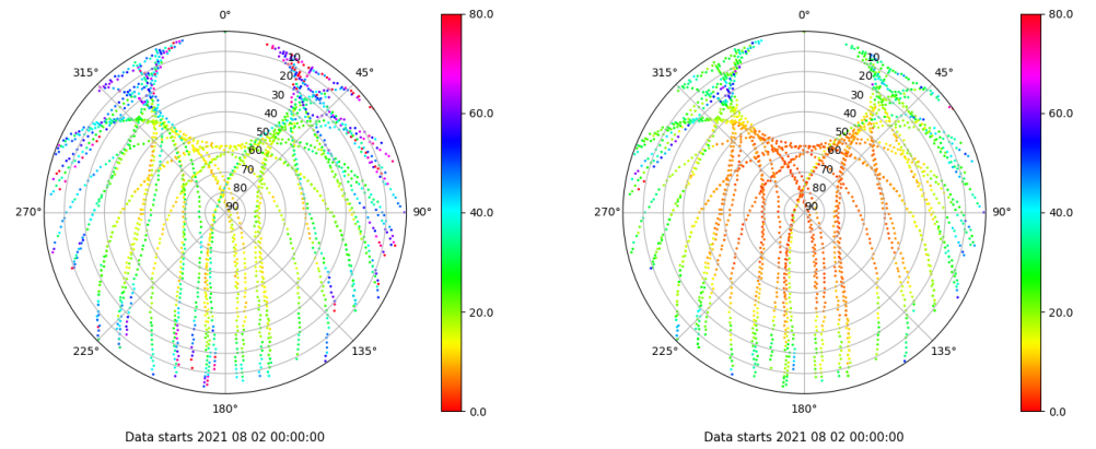
Skyplot for station TALV. Parameter M1C Data file TALV00ESP_R_2021214.xtr Skyplot for station TALV. Parameter M2P Data file TALV00ESP_R_2021214.xtr
