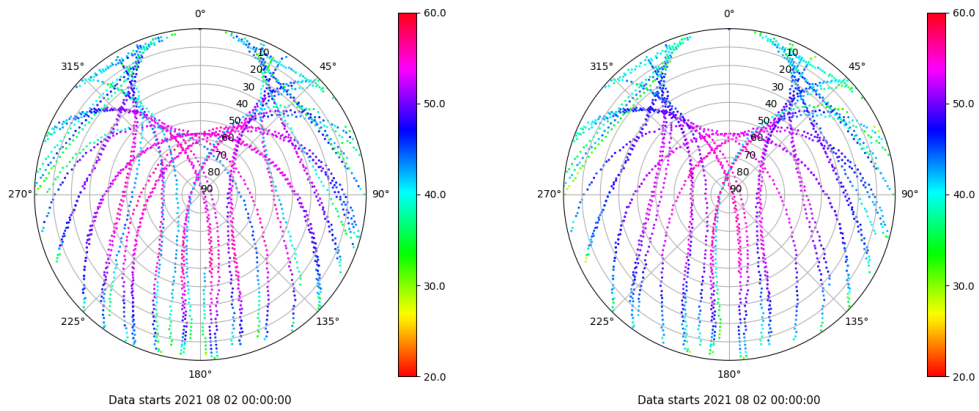
Skyplot for station TALV. Signal to Noise S1C Data file TALV00ESP_R_2021214.xtr Skyplot for station TALV. Signal to Noise S2P Data file TALV00ESP_R_2021214.xtr
