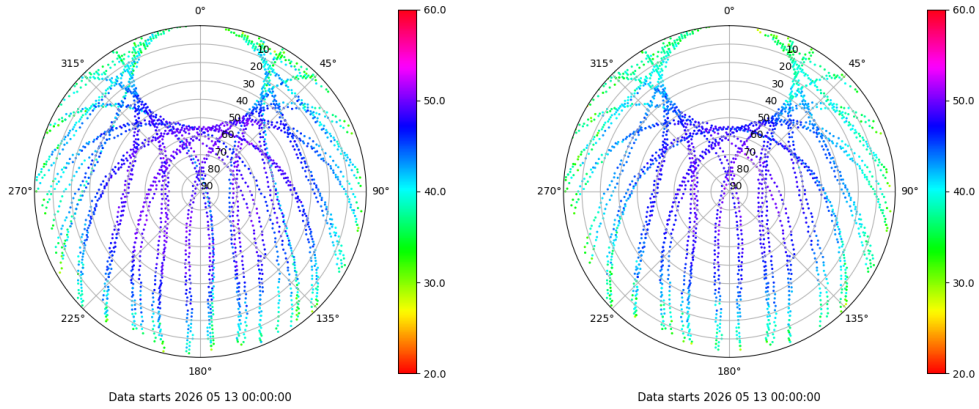
Skyplot for station TALR. Signal to Noise S1C Data file TALR00ESP_R_2026133.xtr Skyplot for station TALR. Signal to Noise S2C Data file TALR00ESP_R_2026133.xtr
