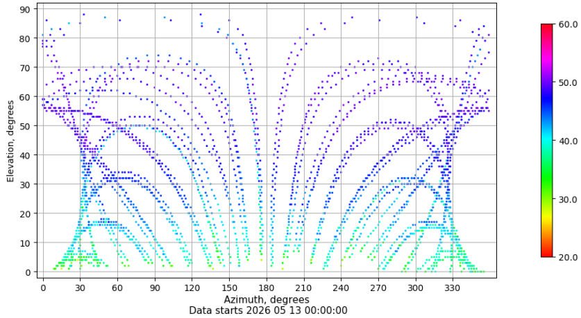
Azimuth-elevation plot for station TALR. Signal to Noise S1C Data file TALR00ESP_R_2026133.xtr
