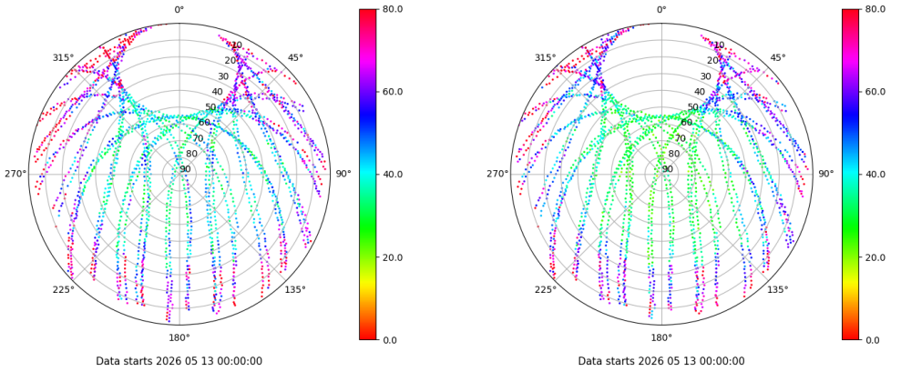
Skyplot for station TALR. Parameter M1C Data file TALR00ESP_R_2026133.xtr Skyplot for station TALR. Parameter M2C Data file TALR00ESP_R_2026133.xtr
