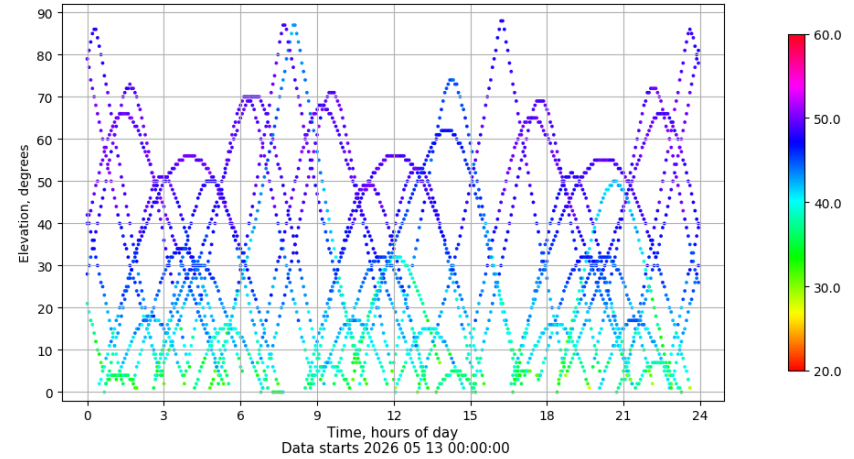
Time-elevation plot for station TALR. Signal to Noise S1C Data file TALR00ESP_R_2026133.xtr
