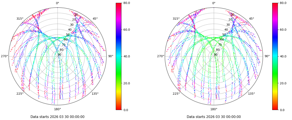
Skyplot for station TALR. Parameter M1C Data file TALR00ESP_R_2026089.xtr Skyplot for station TALR. Parameter M2C Data file TALR00ESP_R_2026089.xtr
