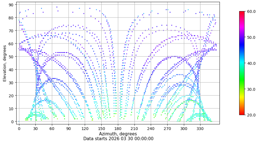
Azimuth-elevation plot for station TALR. Signal to Noise S1C Data file TALR00ESP_R_2026089.xtr
