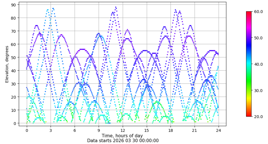
Time-elevation plot for station TALR. Signal to Noise S1C Data file TALR00ESP_R_2026089.xtr
