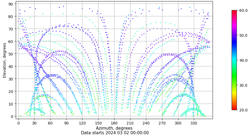
Azimuth-elevation plot for station TALR. Signal to Noise S1C Data file TALR00ESP_R_2024062.xtr
