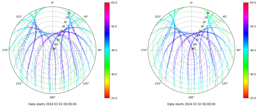
Skyplot for station TALR. Signal to Noise S1C Data file TALR00ESP_R_2024062.xtr Skyplot for station TALR. Signal to Noise S2C Data file TALR00ESP_R_2024062.xtr
