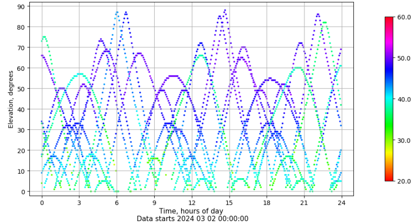
Time-elevation plot for station TALR. Signal to Noise S1C Data file TALR00ESP_R_2024062.xtr
