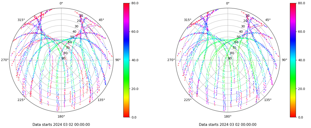
Skyplot for station TALR. Parameter M1C Data file TALR00ESP_R_2024062.xtr Skyplot for station TALR. Parameter M2C Data file TALR00ESP_R_2024062.xtr
