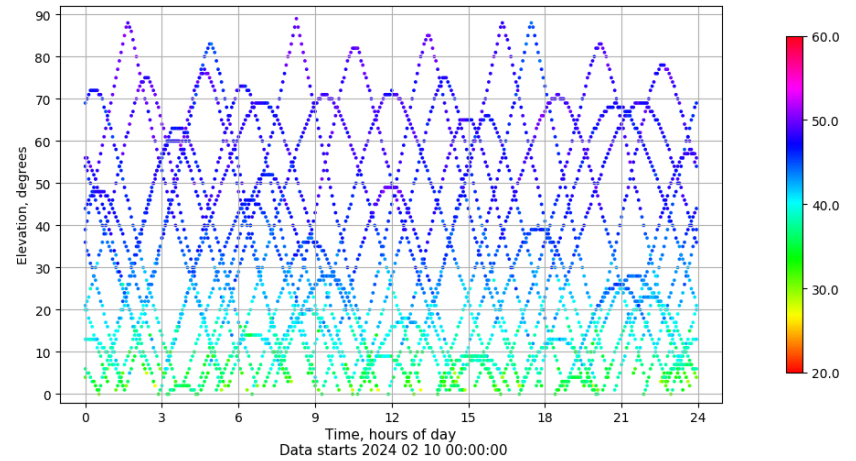
Time-elevation plot for station TALR. Signal to Noise S1C Data file TALR00ESP_R_2024041.xtr
