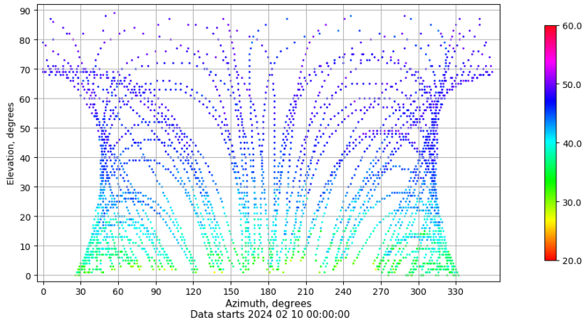
Azimuth-elevation plot for station TALR. Signal to Noise S1C Data file TALR00ESP_R_2024041.xtr
