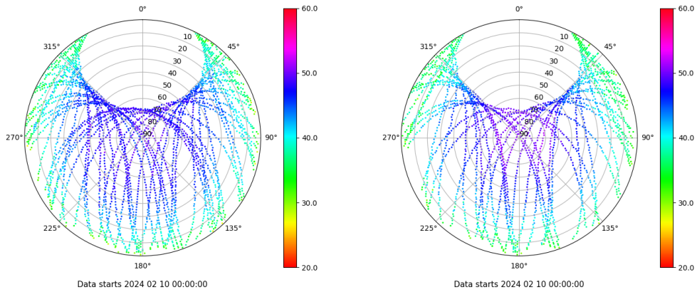
Skyplot for station TALR. Signal to Noise S1C Data file TALR00ESP_R_2024041.xtr Skyplot for station TALR. Signal to Noise S2X Data file TALR00ESP_R_2024041.xtr
