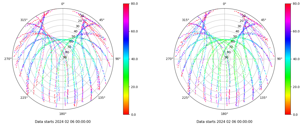
Skyplot for station TALR. Parameter M1C Data file TALR00ESP_R_2024037.xtr Skyplot for station TALR. Parameter M2C Data file TALR00ESP_R_2024037.xtr
