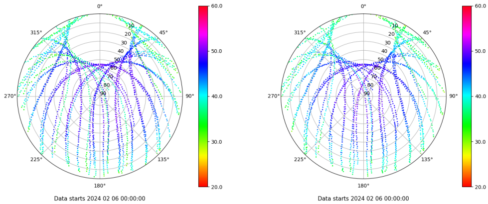
Skyplot for station TALR. Signal to Noise S1C Data file TALR00ESP_R_2024037.xtr Skyplot for station TALR. Signal to Noise S2C Data file TALR00ESP_R_2024037.xtr
