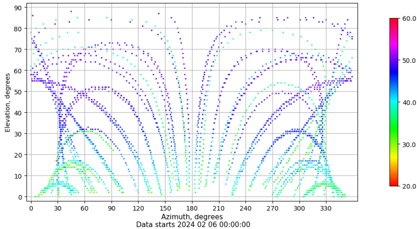
Azimuth-elevation plot for station TALR. Signal to Noise S1C Data file TALR00ESP_R_2024037.xtr
