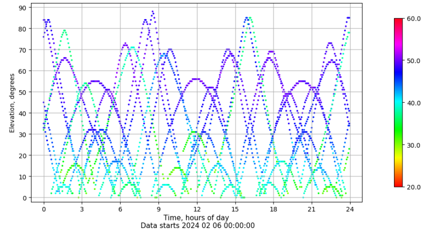
Time-elevation plot for station TALR. Signal to Noise S1C Data file TALR00ESP_R_2024037.xtr
