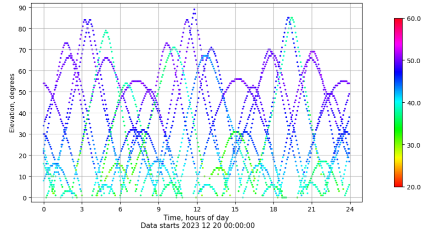
Time-elevation plot for station TALR. Signal to Noise S1C Data file TALR00ESP_R_2023354.xtr
