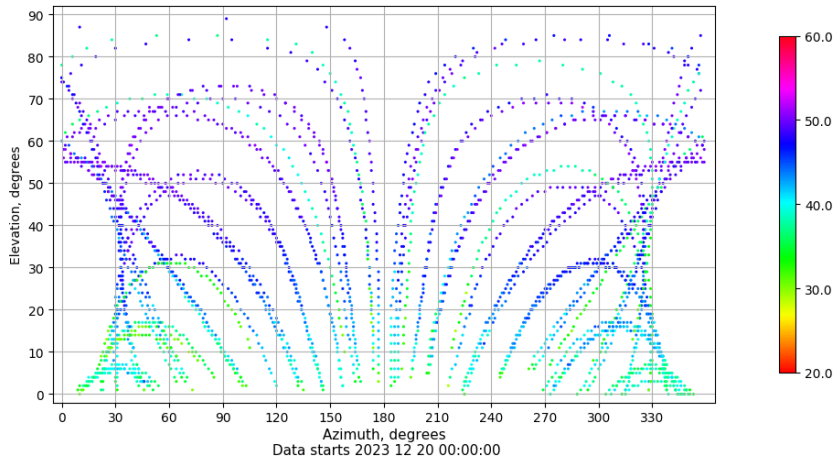
Azimuth-elevation plot for station TALR. Signal to Noise S1C Data file TALR00ESP_R_2023354.xtr
