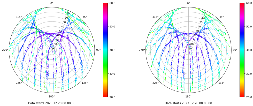
Skyplot for station TALR. Signal to Noise S1C Data file TALR00ESP_R_2023354.xtr Skyplot for station TALR. Signal to Noise S2C Data file TALR00ESP_R_2023354.xtr
