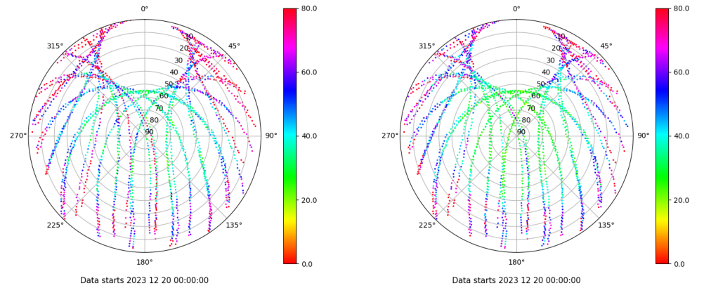
Skyplot for station TALR. Parameter M1C Data file TALR00ESP_R_2023354.xtr Skyplot for station TALR. Parameter M2C Data file TALR00ESP_R_2023354.xtr
