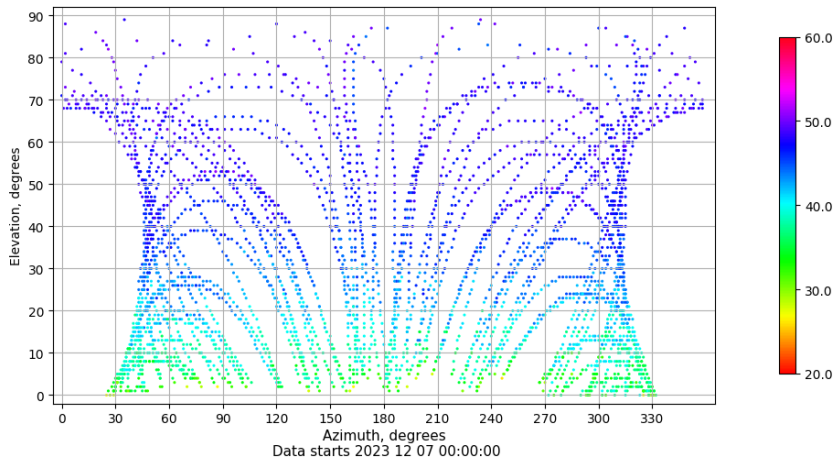
Azimuth-elevation plot for station TALR. Signal to Noise S1C Data file TALR00ESP_R_2023341.xtr
