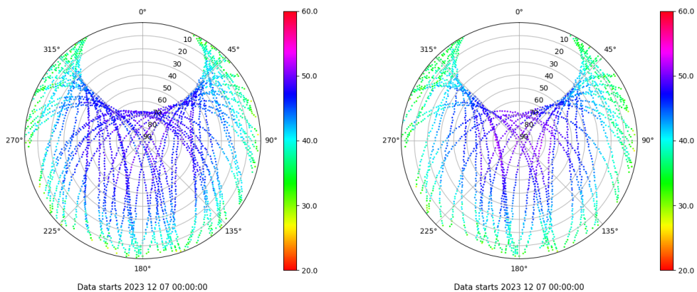
Skyplot for station TALR. Signal to Noise S1C Data file TALR00ESP_R_2023341.xtr Skyplot for station TALR. Signal to Noise S2X Data file TALR00ESP_R_2023341.xtr
