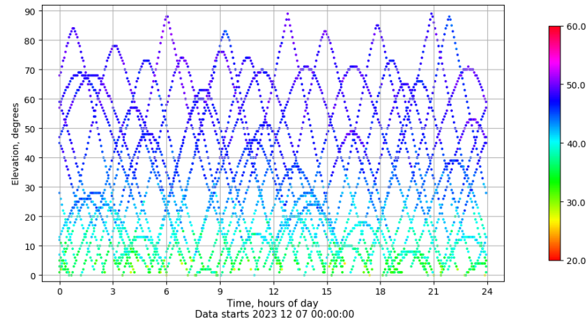
Time-elevation plot for station TALR. Signal to Noise S1C Data file TALR00ESP_R_2023341.xtr
