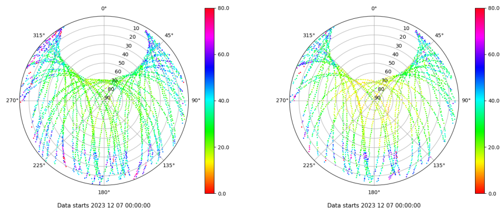
Skyplot for station TALR. Parameter M1C Data file TALR00ESP_R_2023341.xtr Skyplot for station TALR. Parameter M2X Data file TALR00ESP_R_2023341.xtr
