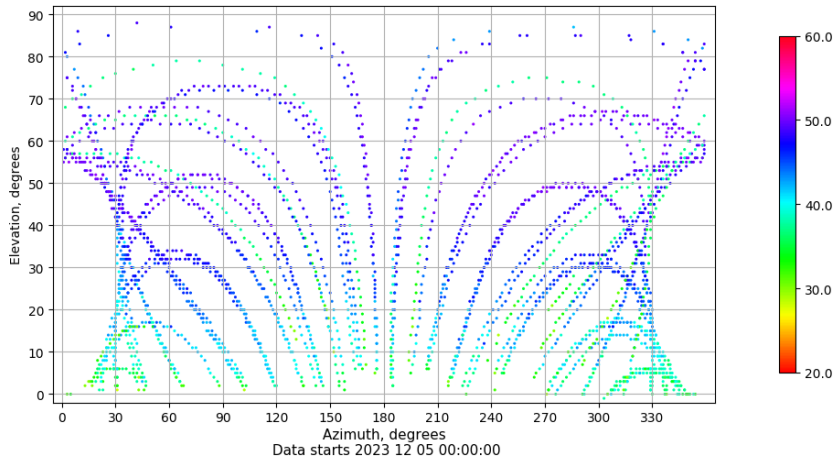
Azimuth-elevation plot for station TALR. Signal to Noise S1C Data file TALR00ESP_R_2023339.xtr
