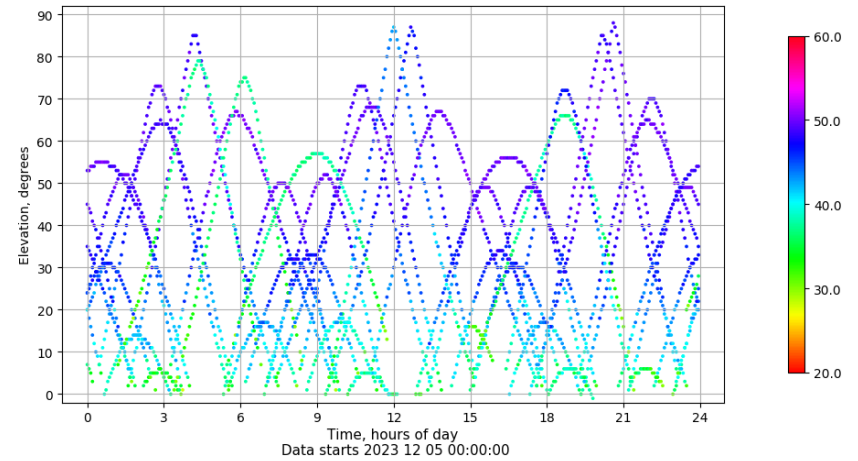
Time-elevation plot for station TALR. Signal to Noise S1C Data file TALR00ESP_R_2023339.xtr
