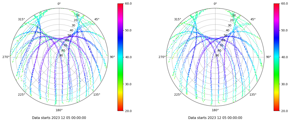
Skyplot for station TALR. Signal to Noise S1C Data file TALR00ESP_R_2023339.xtr Skyplot for station TALR. Signal to Noise S2C Data file TALR00ESP_R_2023339.xtr
