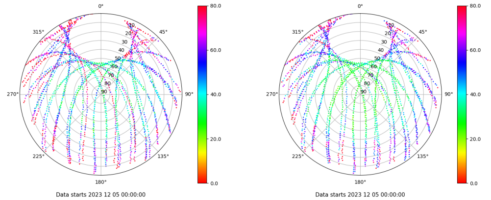
Skyplot for station TALR. Parameter M1C Data file TALR00ESP_R_2023339.xtr Skyplot for station TALR. Parameter M2C Data file TALR00ESP_R_2023339.xtr
