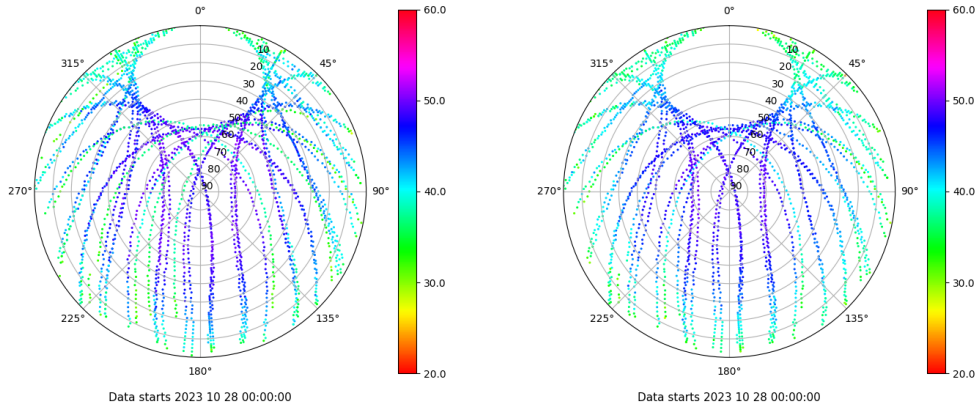
Skyplot for station TALR. Signal to Noise S1C Data file TALR00ESP_R_2023301.xtr Skyplot for station TALR. Signal to Noise S2C Data file TALR00ESP_R_2023301.xtr
