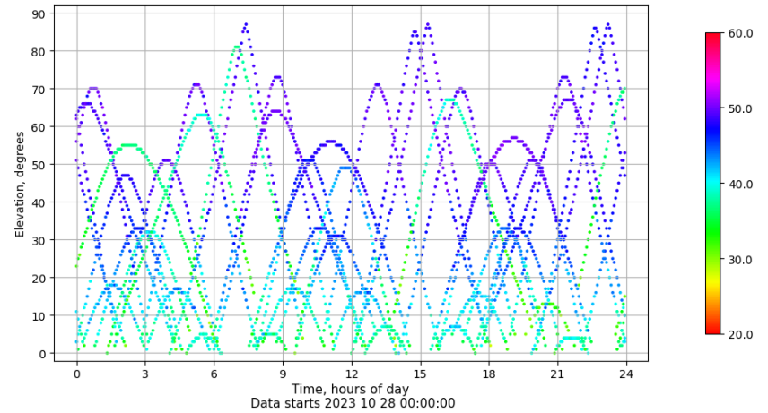
Time-elevation plot for station TALR. Signal to Noise S1C Data file TALR00ESP_R_2023301.xtr
