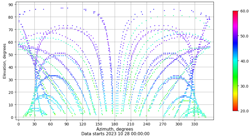
Azimuth-elevation plot for station TALR. Signal to Noise S1C Data file TALR00ESP_R_2023301.xtr
