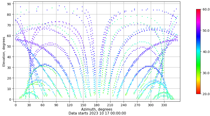
Azimuth-elevation plot for station TALR. Signal to Noise S1C Data file TALR00ESP_R_2023290.xtr
