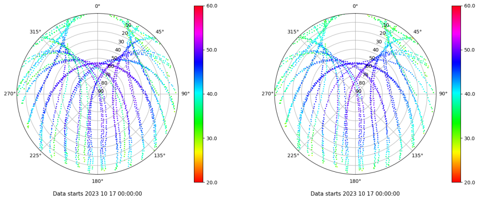
Skyplot for station TALR. Signal to Noise S1C Data file TALR00ESP_R_2023290.xtr Skyplot for station TALR. Signal to Noise S2C Data file TALR00ESP_R_2023290.xtr
