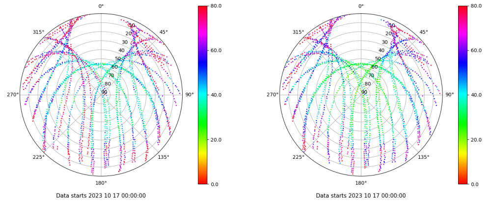
Skyplot for station TALR. Parameter M1C Data file TALR00ESP_R_2023290.xtr Skyplot for station TALR. Parameter M2C Data file TALR00ESP_R_2023290.xtr
