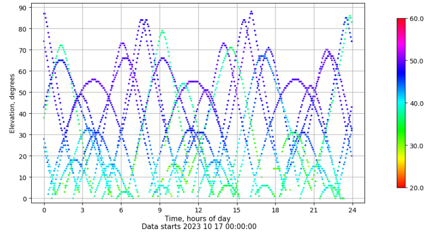
Time-elevation plot for station TALR. Signal to Noise S1C Data file TALR00ESP_R_2023290.xtr
