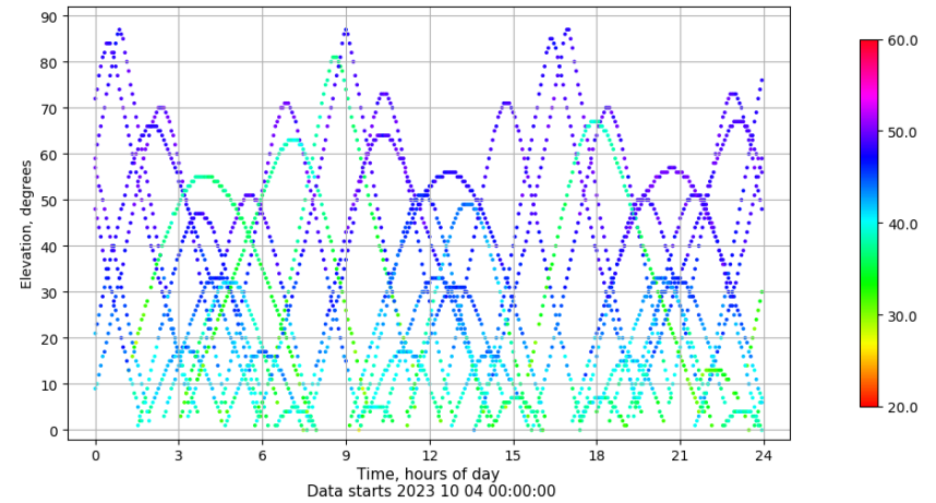
Time-elevation plot for station TALR. Signal to Noise S1C Data file TALR00ESP_R_2023277.xtr
