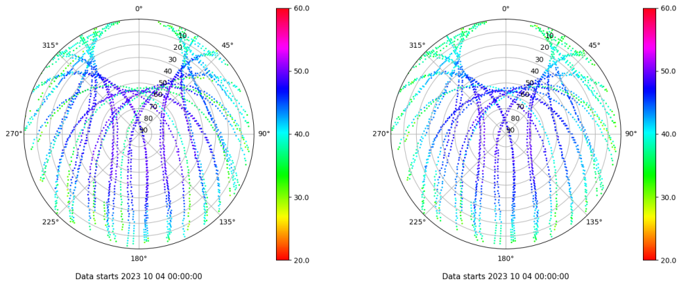
Skyplot for station TALR. Signal to Noise S1C Data file TALR00ESP_R_2023277.xtr Skyplot for station TALR. Signal to Noise S2C Data file TALR00ESP_R_2023277.xtr
