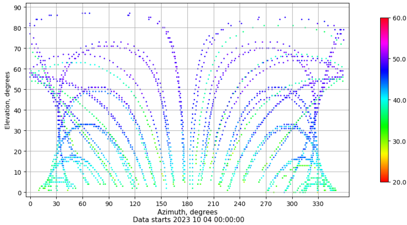
Azimuth-elevation plot for station TALR. Signal to Noise S1C Data file TALR00ESP_R_2023277.xtr
