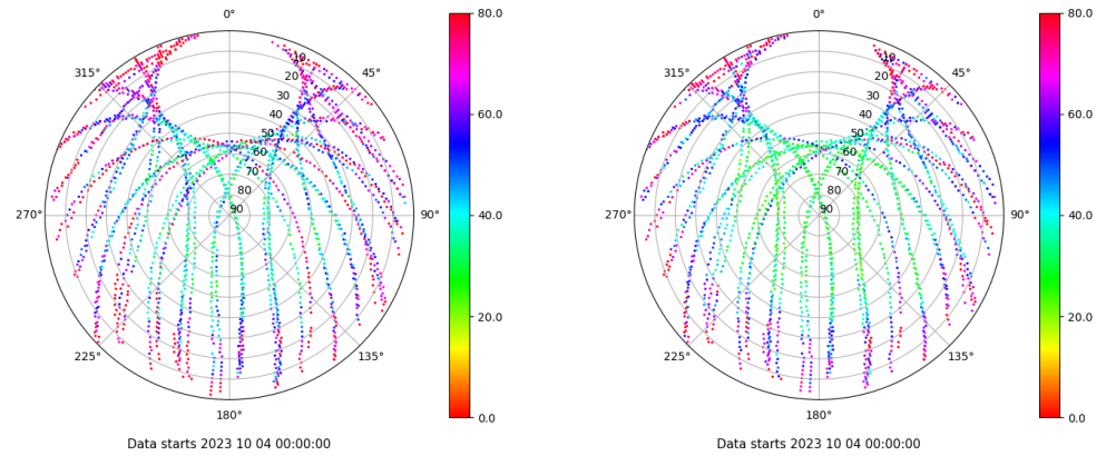
Skyplot for station TALR. Parameter M1C Data file TALR00ESP_R_2023277.xtr Skyplot for station TALR. Parameter M2C Data file TALR00ESP_R_2023277.xtr
