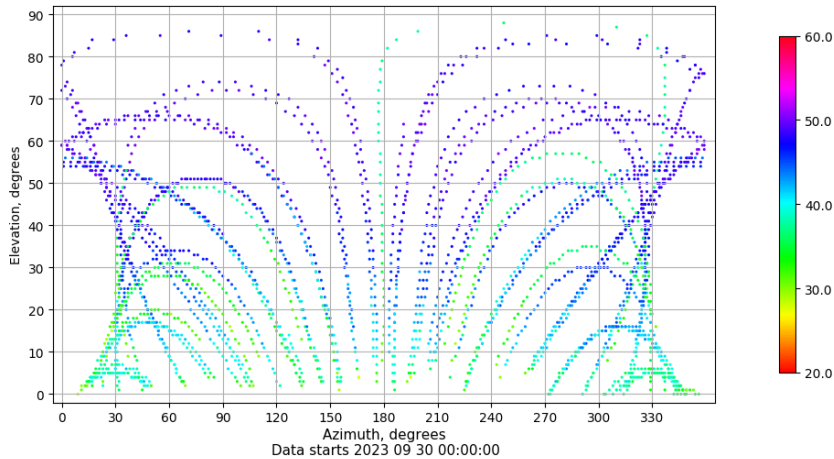
Azimuth-elevation plot for station TALR. Signal to Noise S1C Data file TALR00ESP_R_2023273.xtr
