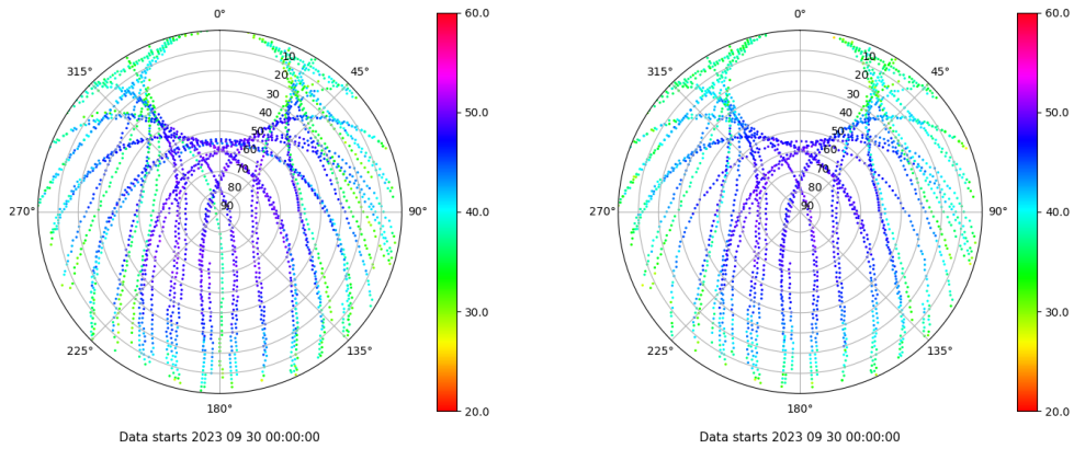
Skyplot for station TALR. Signal to Noise S1C Data file TALR00ESP_R_2023273.xtr Skyplot for station TALR. Signal to Noise S2C Data file TALR00ESP_R_2023273.xtr
