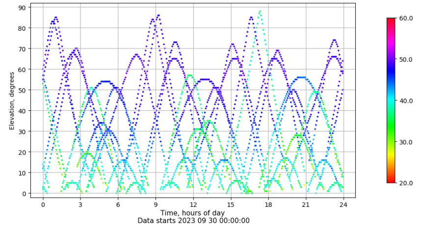
Time-elevation plot for station TALR. Signal to Noise S1C Data file TALR00ESP_R_2023273.xtr
