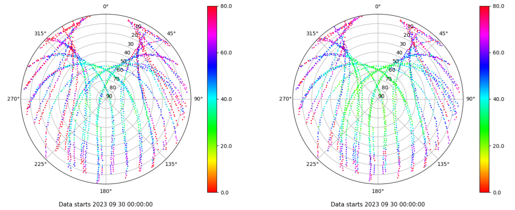
Skyplot for station TALR. Parameter M1C Data file TALR00ESP_R_2023273.xtr Skyplot for station TALR. Parameter M2C Data file TALR00ESP_R_2023273.xtr
