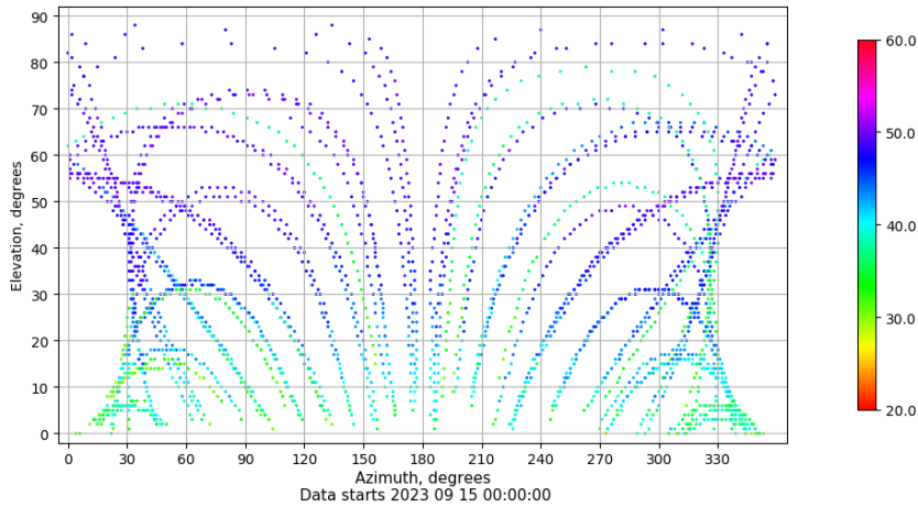
Azimuth-elevation plot for station TALR. Signal to Noise S1C Data file TALR00ESP_R_2023258.xtr
