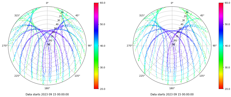
Skyplot for station TALR. Signal to Noise S1C Data file TALR00ESP_R_2023258.xtr Skyplot for station TALR. Signal to Noise S2C Data file TALR00ESP_R_2023258.xtr
