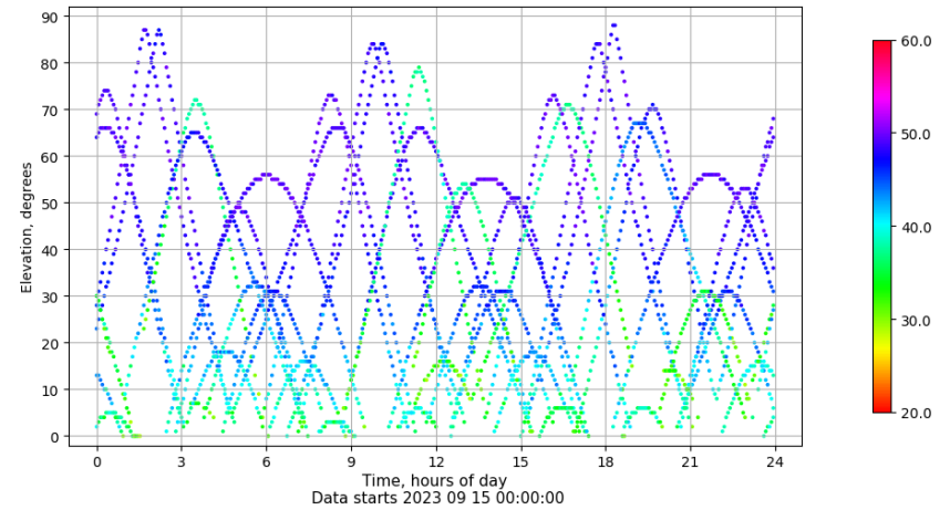
Time-elevation plot for station TALR. Signal to Noise S1C Data file TALR00ESP_R_2023258.xtr
