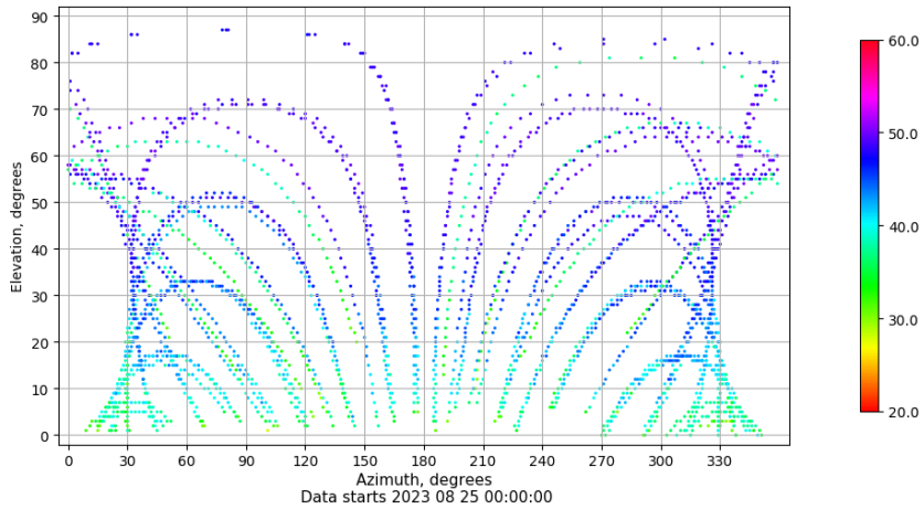
Azimuth-elevation plot for station TALR. Signal to Noise S1C Data file TALR00ESP_R_2023237.xtr
