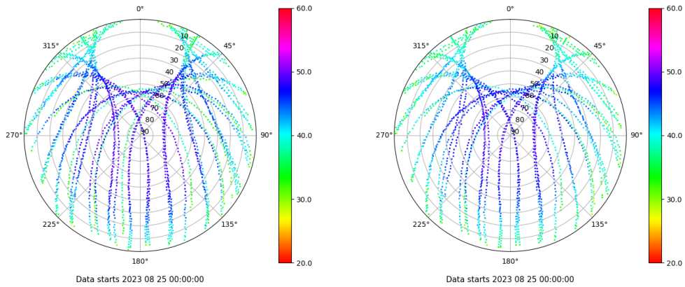
Skyplot for station TALR. Signal to Noise S1C Data file TALR00ESP_R_2023237.xtr Skyplot for station TALR. Signal to Noise S2C Data file TALR00ESP_R_2023237.xtr
