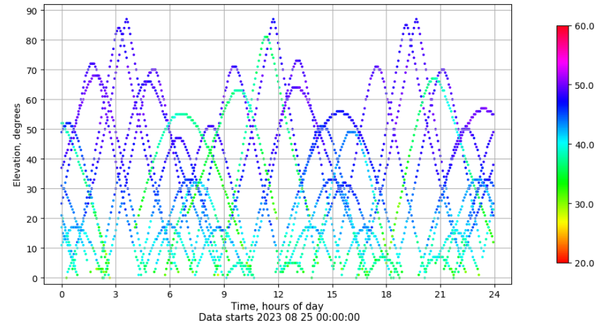
Time-elevation plot for station TALR. Signal to Noise S1C Data file TALR00ESP_R_2023237.xtr
