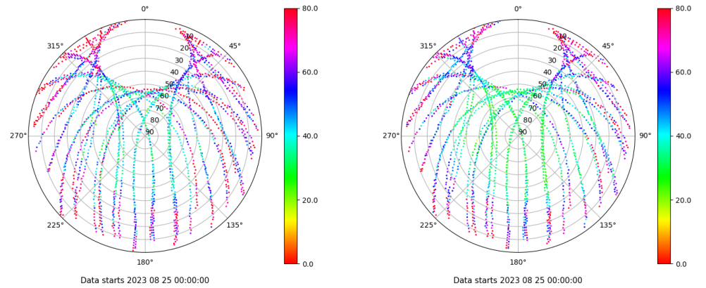
Skyplot for station TALR. Parameter M1C Data file TALR00ESP_R_2023237.xtr Skyplot for station TALR. Parameter M2C Data file TALR00ESP_R_2023237.xtr
